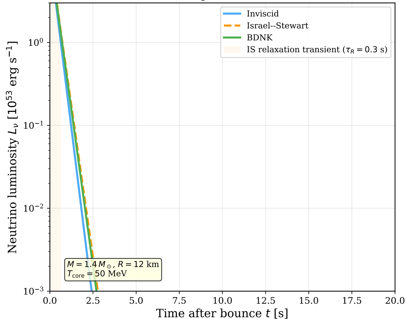
Proto-NS neutrino signal: BDNK vs IS vs inviscid
