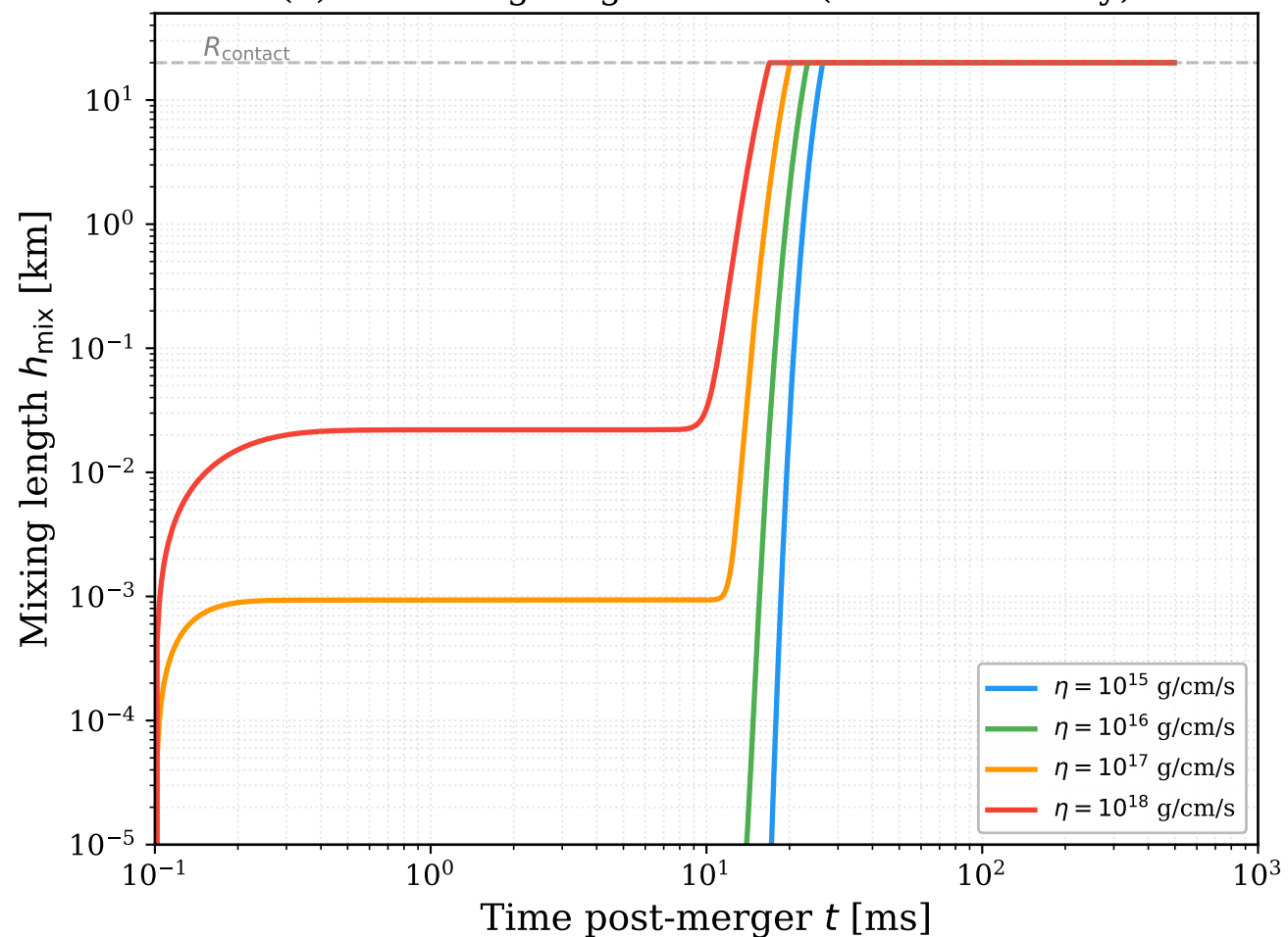
(a) RT mixing length vs time (BDNK viscosity)
