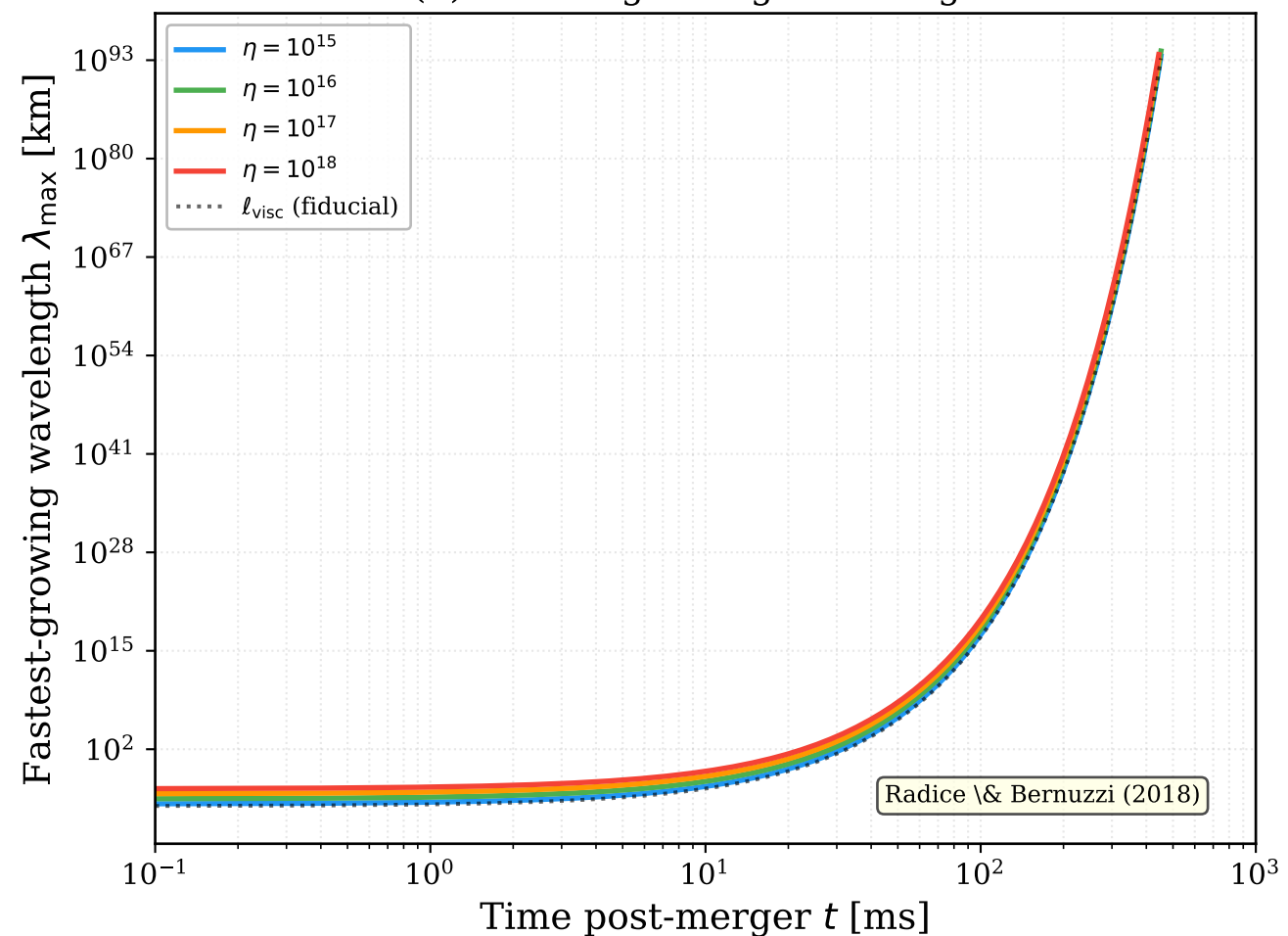
(b) Fastest-growing wavelength
