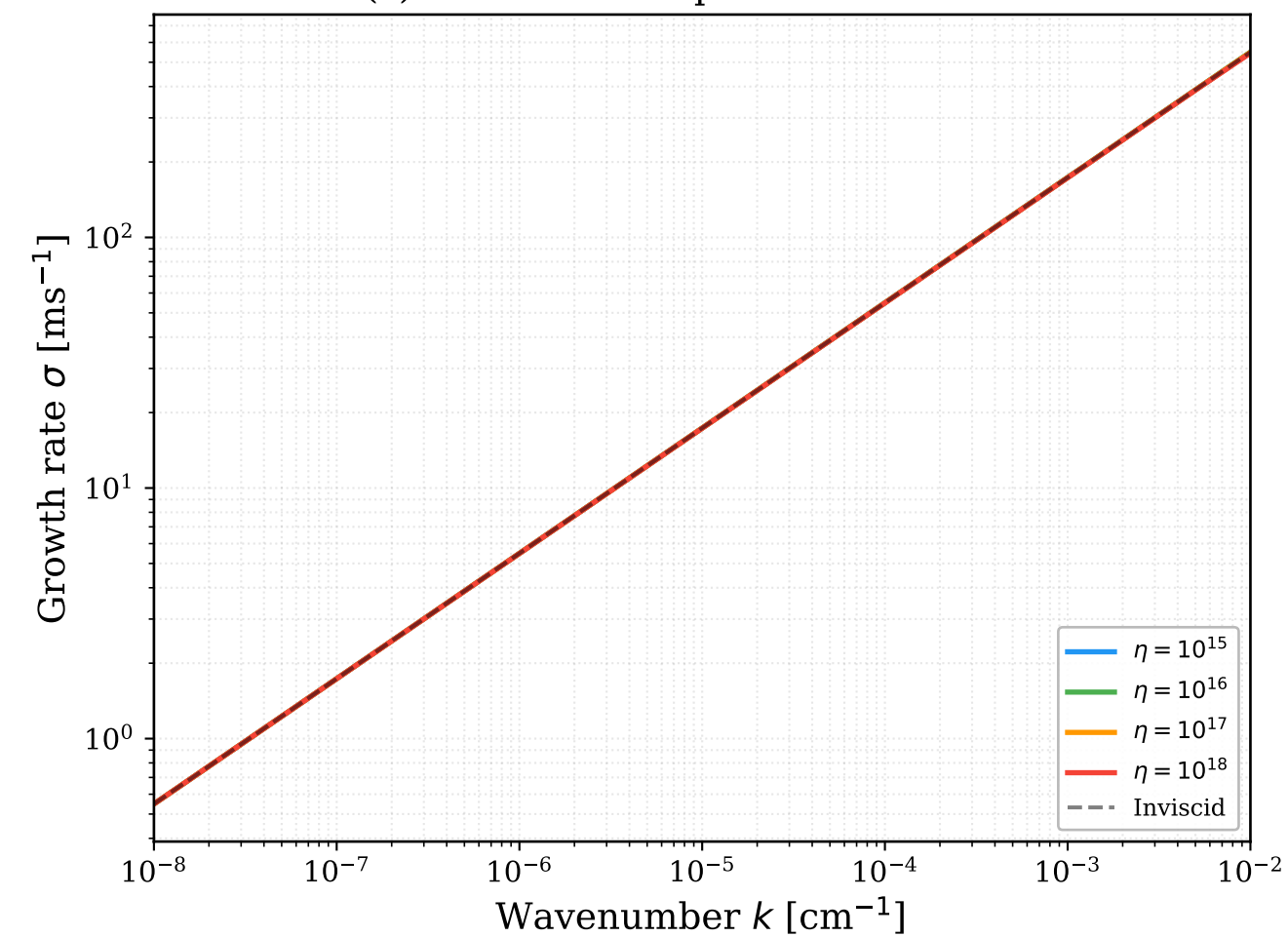
(c) Viscous RT dispersion at t = 1 ms
