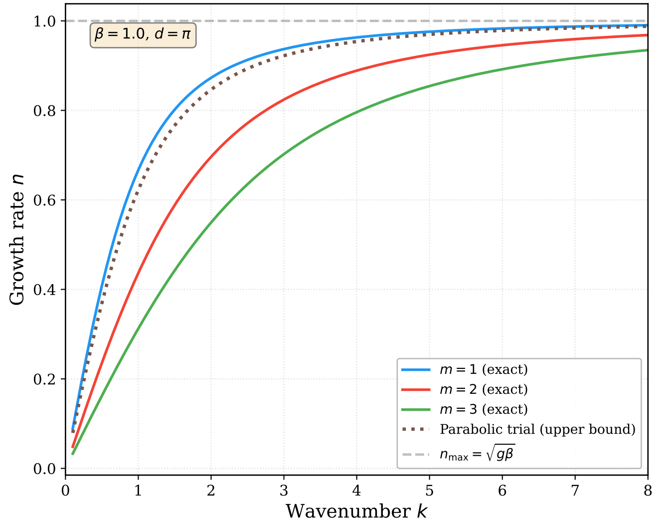
RT growth: exact modes and variational bounds
