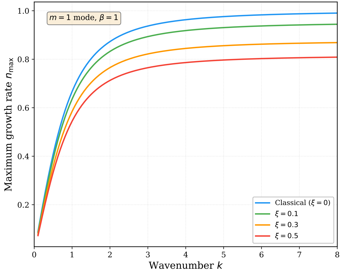
Variational bound: relativistic correction
