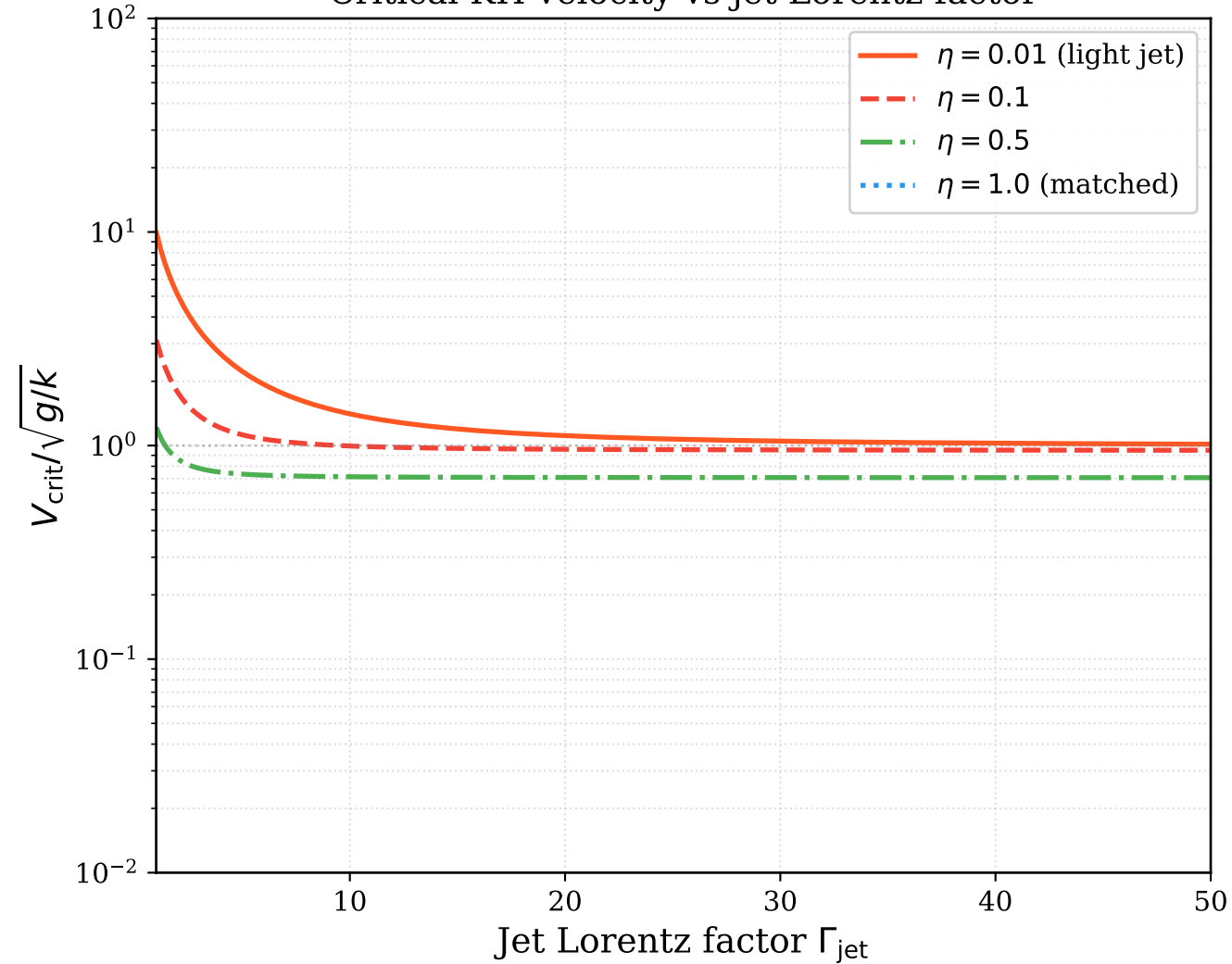
Critical KH velocity vs jet Lorentz factor
