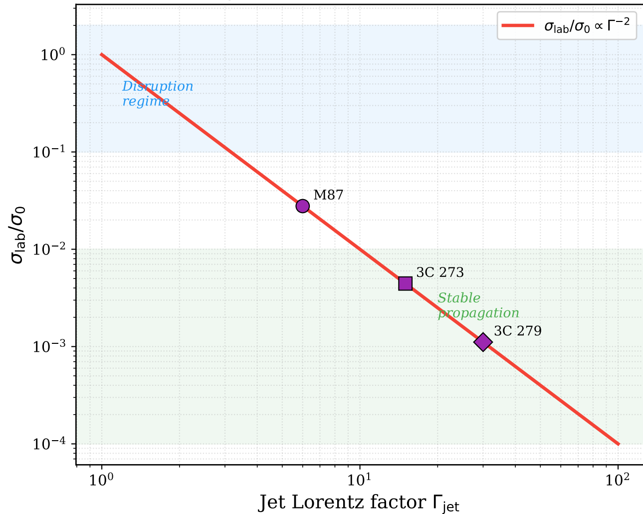
KH growth rate suppression: \sigma \propto \Gamma^{-2}
