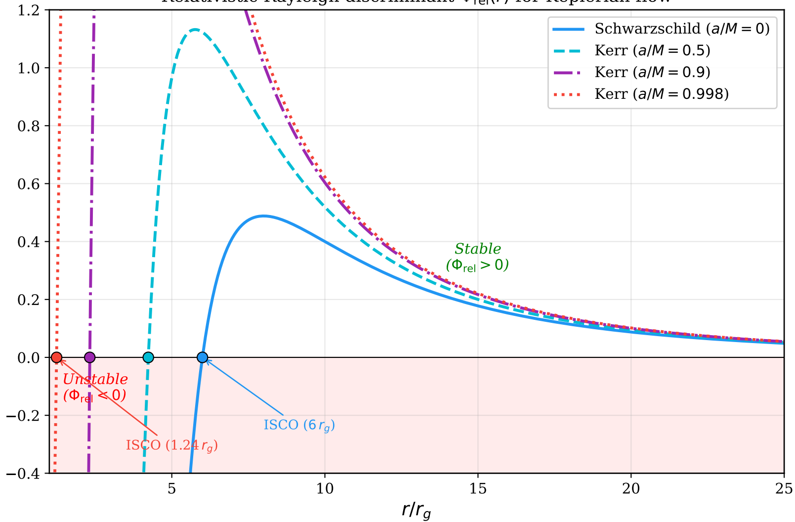
Relativistic Rayleigh discriminant \Phi_{\text{rel}}(r) for Keplerian flow
