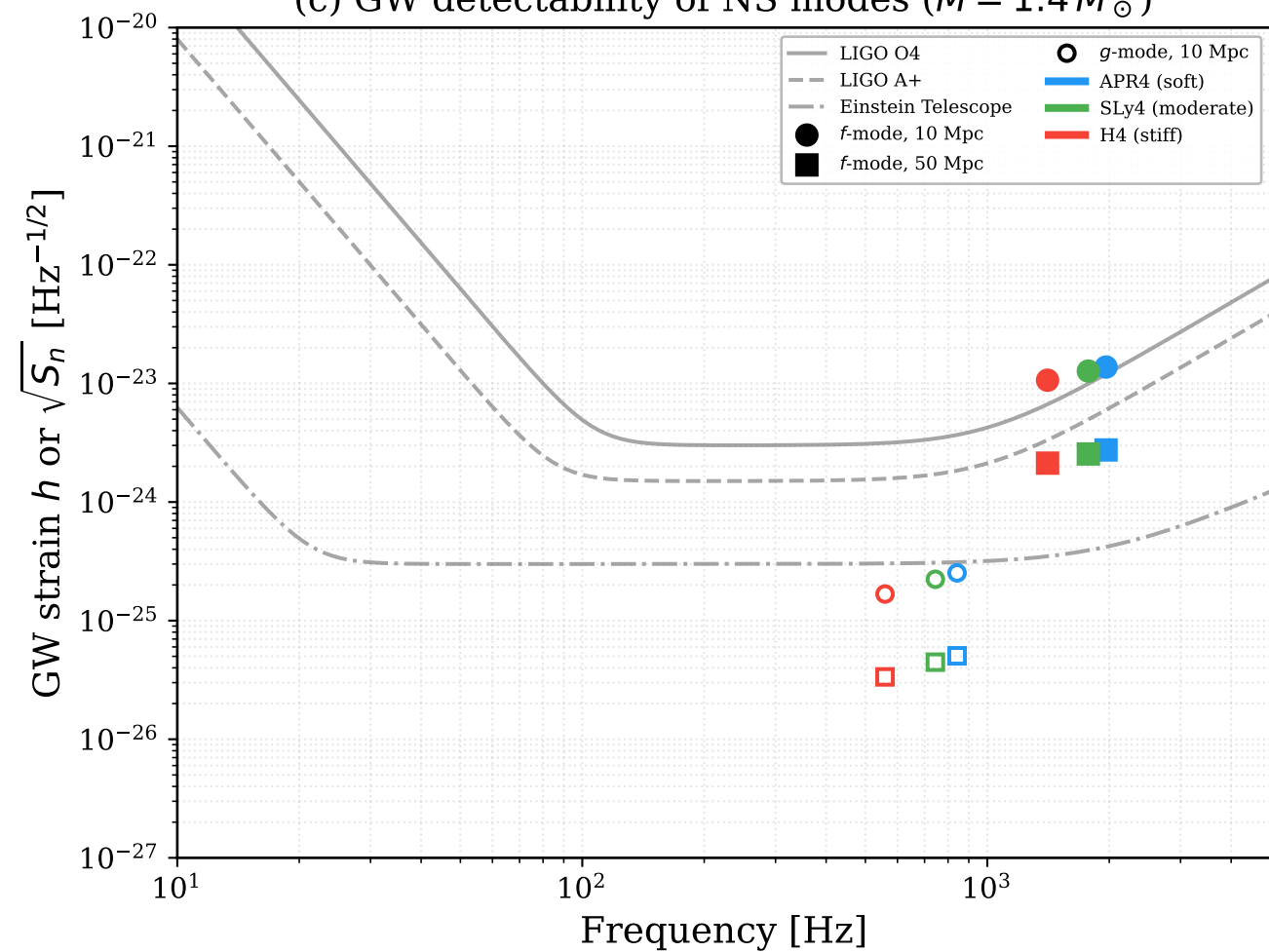
(c) GW detectability of NS modes ( M = 1.4 M_\odot )
