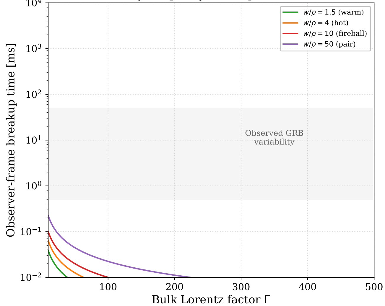
GRB jet capillary breakup timescale
