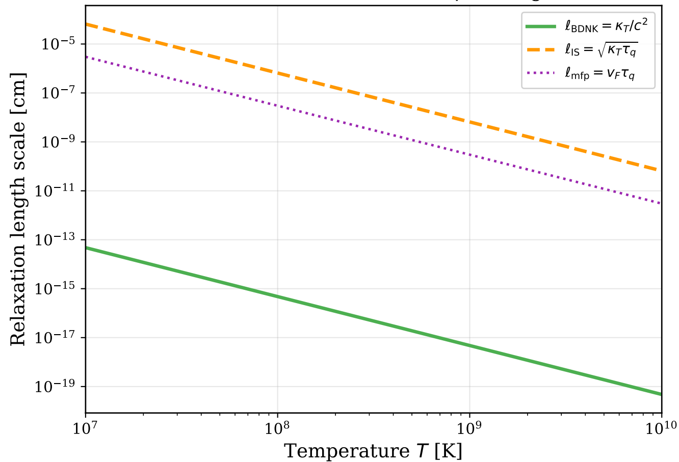
Thermal relaxation: NS ocean ( \rho = 10^9 \text{ g/cm}^3 )
