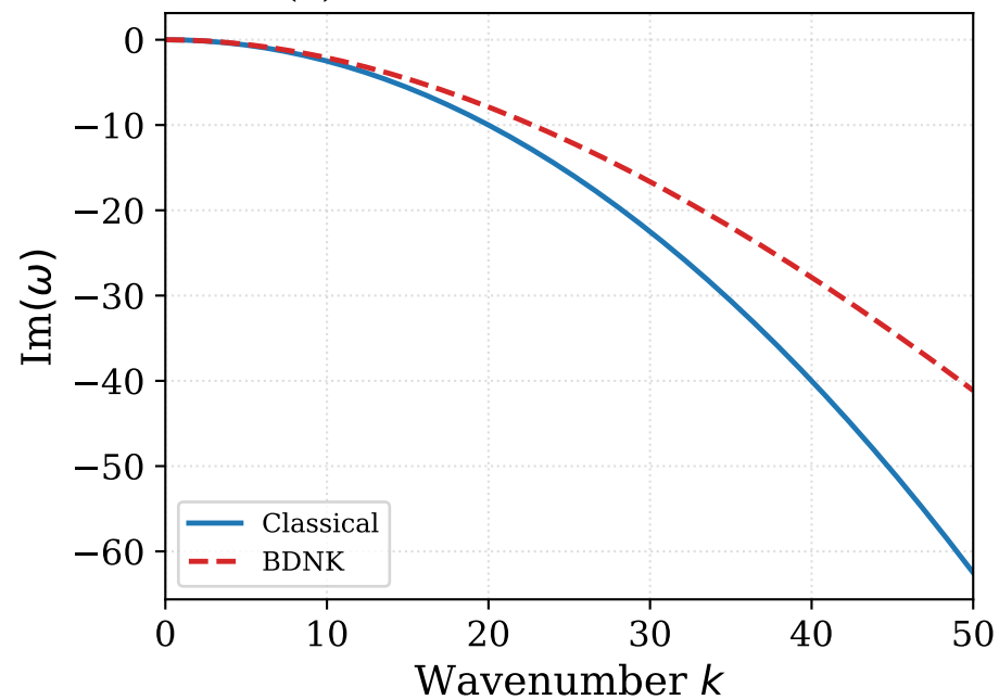
(c) Sound mode attenuation
