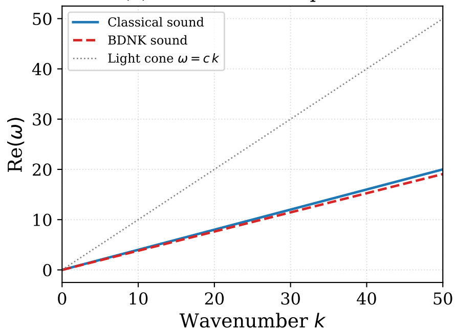
(a) Sound mode dispersion
