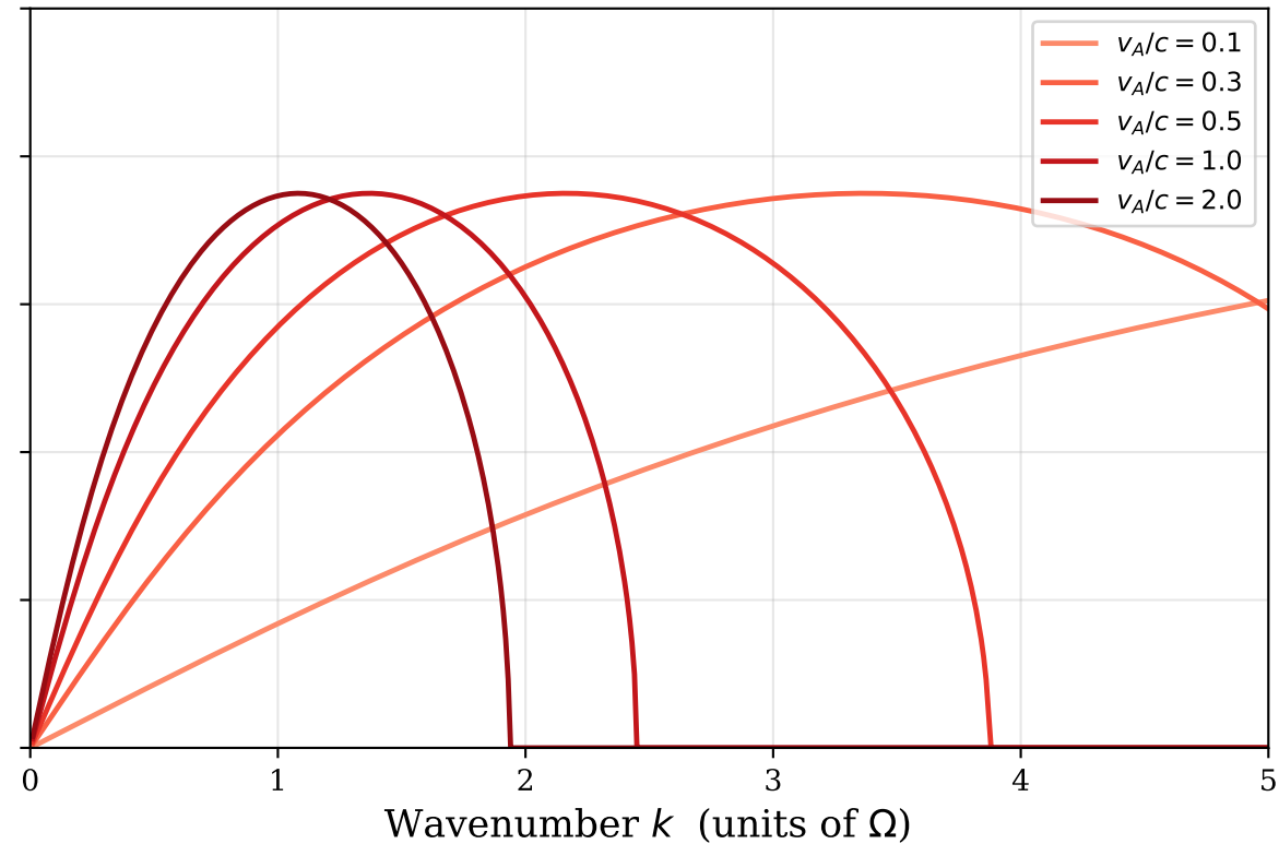
Relativistic MRI (bounded Alfvén speed)
