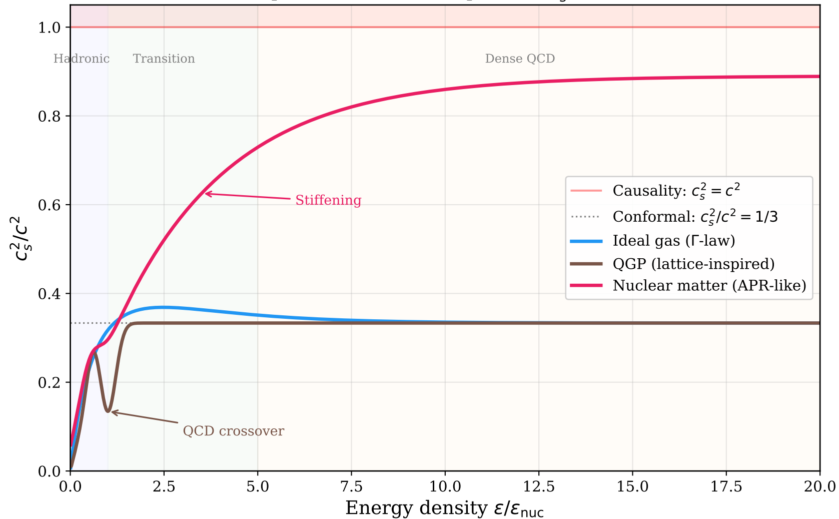
Equation of State Comparison: c_s^2/c^2 vs \varepsilon
