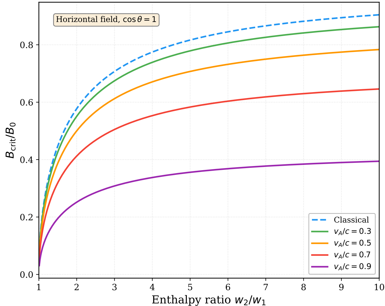
Critical B-field for RT stabilization
