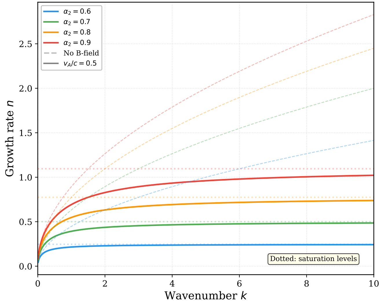
RT with vertical B-field: growth rate saturation
