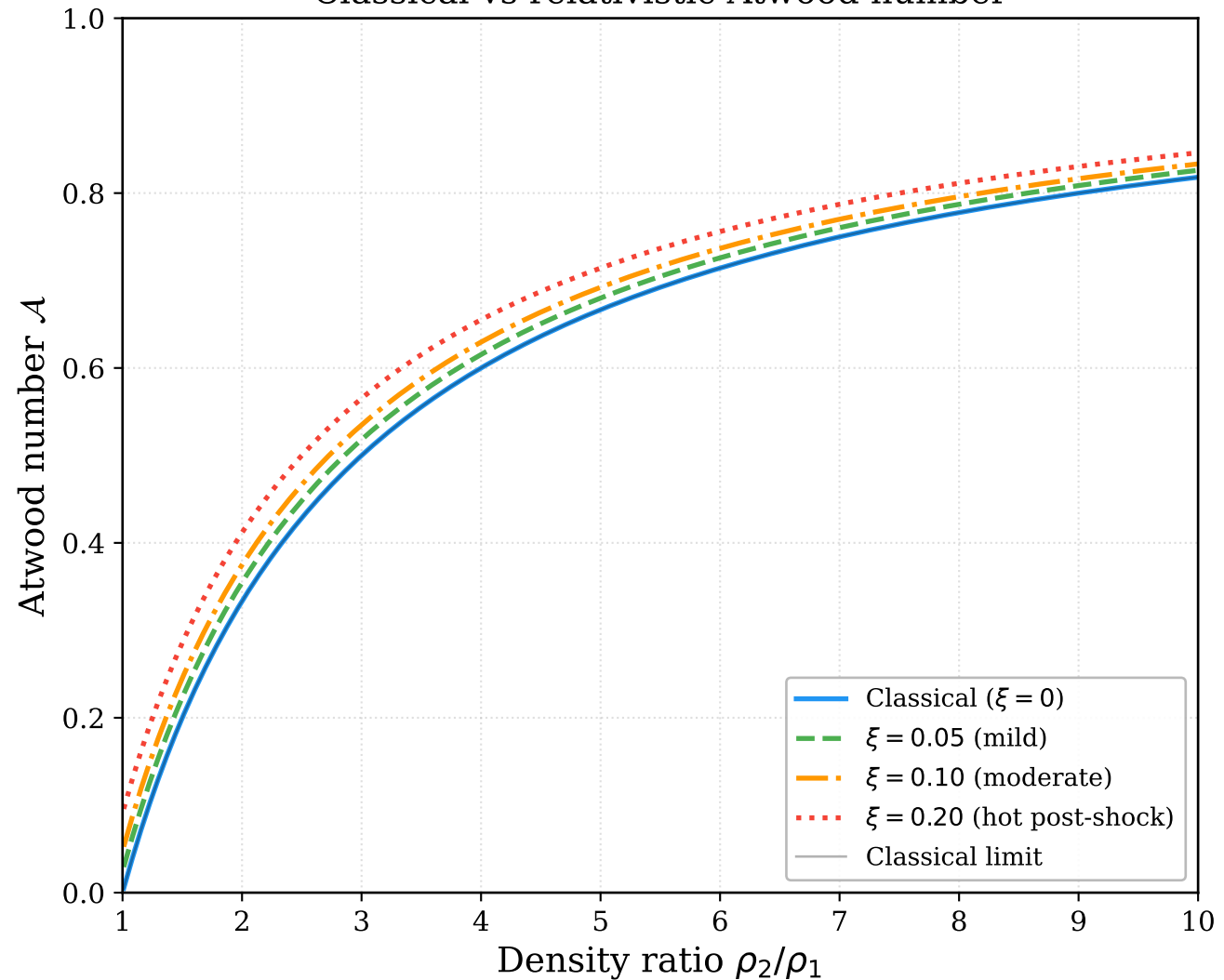
Classical vs relativistic Atwood number
