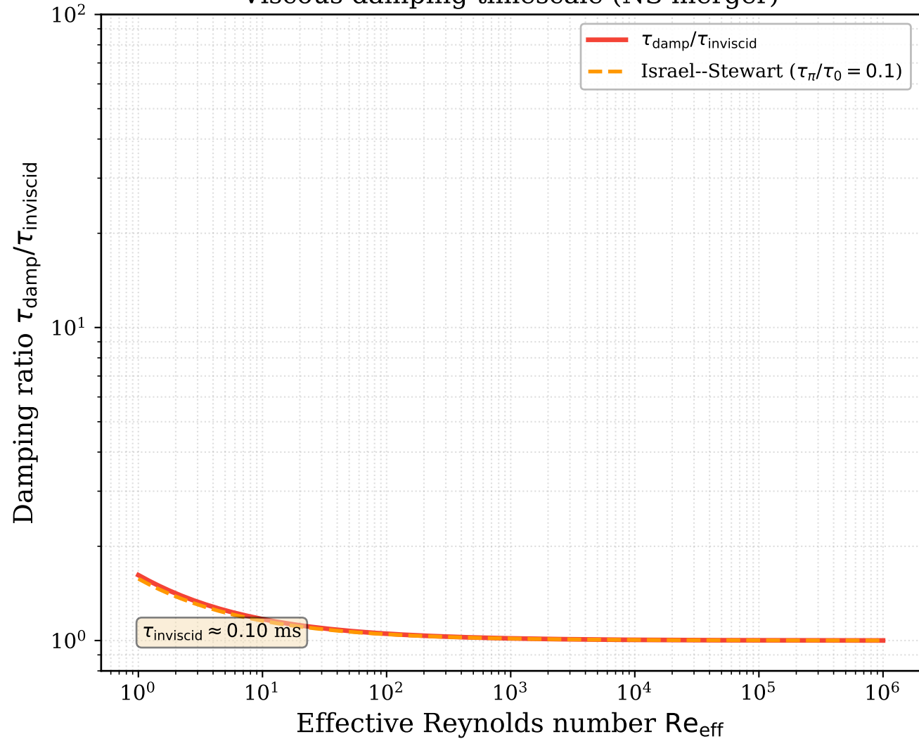
Viscous damping timescale (NS merger)
