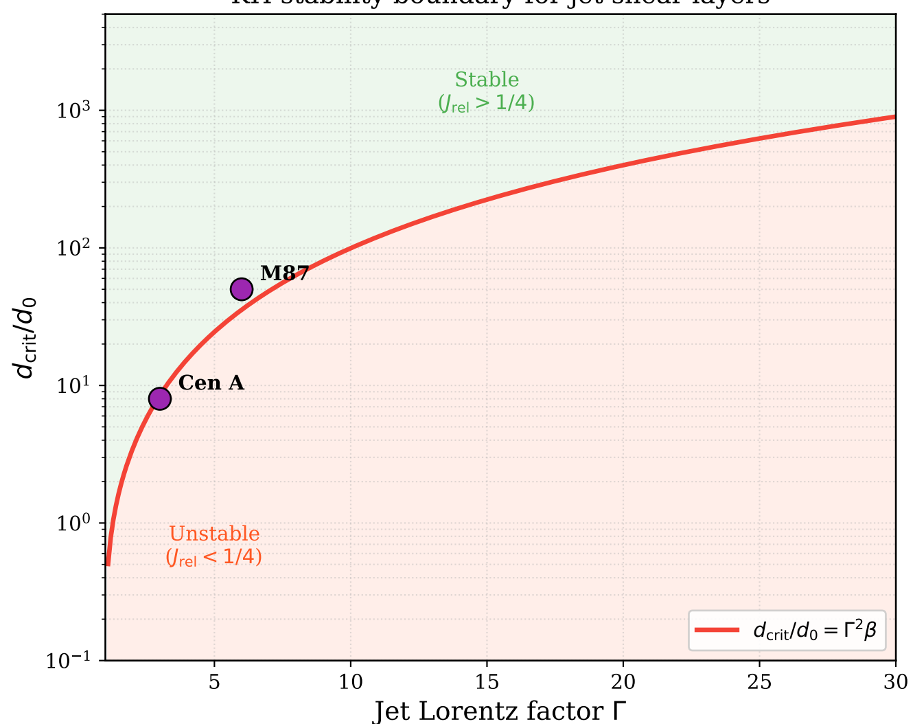
KH stability boundary for jet shear layers
