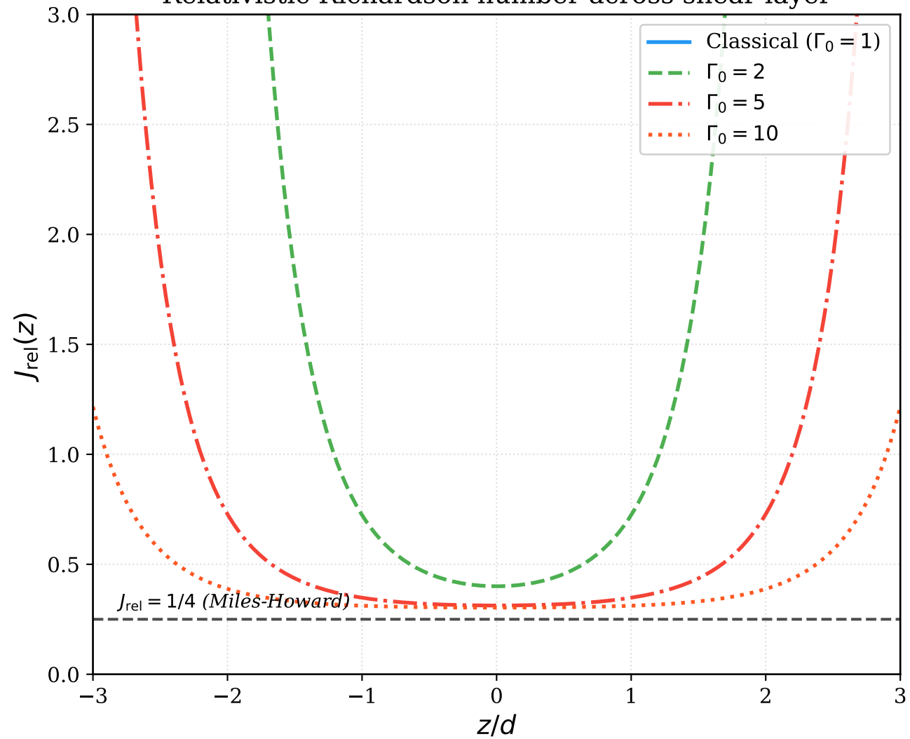
Relativistic Richardson number across shear layer
