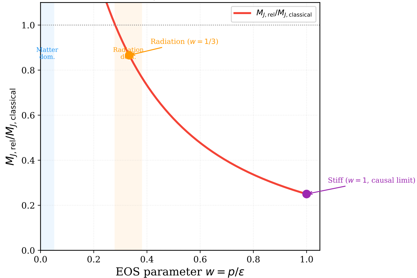
Relativistic Jeans mass reduction
