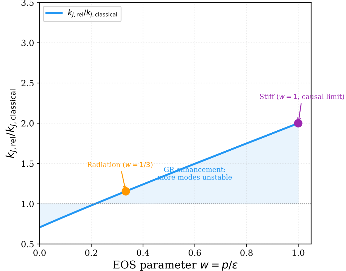
Relativistic Jeans wavenumber enhancement
