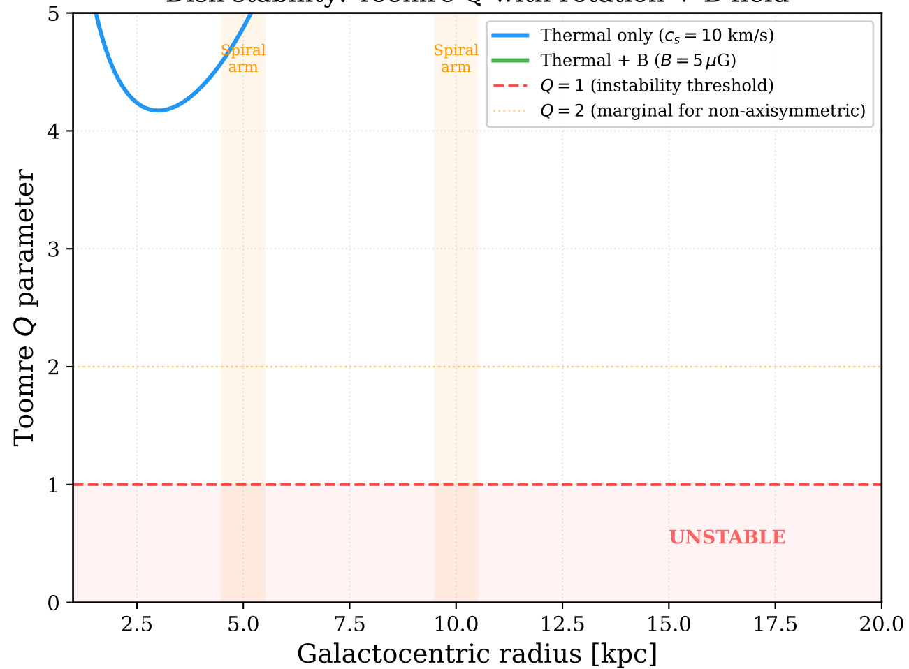
Disk stability: Toomre Q with rotation + B field
