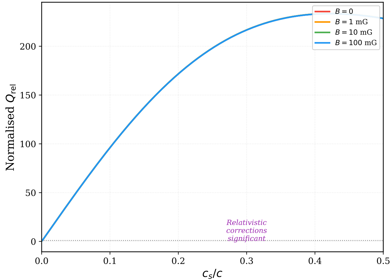
Relativistic Q vs sound speed (compact disk)
