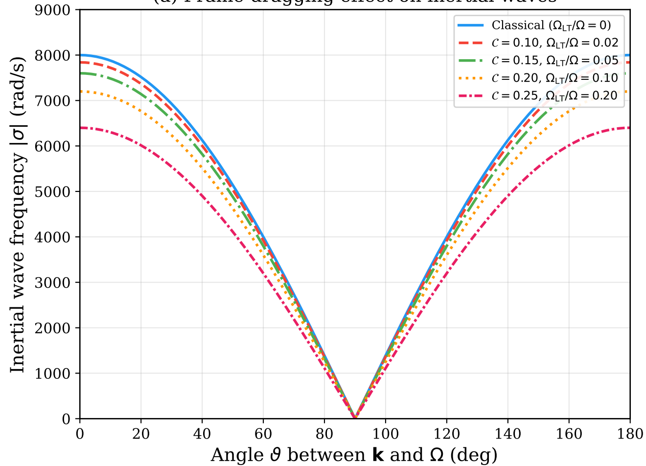
(a) Frame-dragging effect on inertial waves
