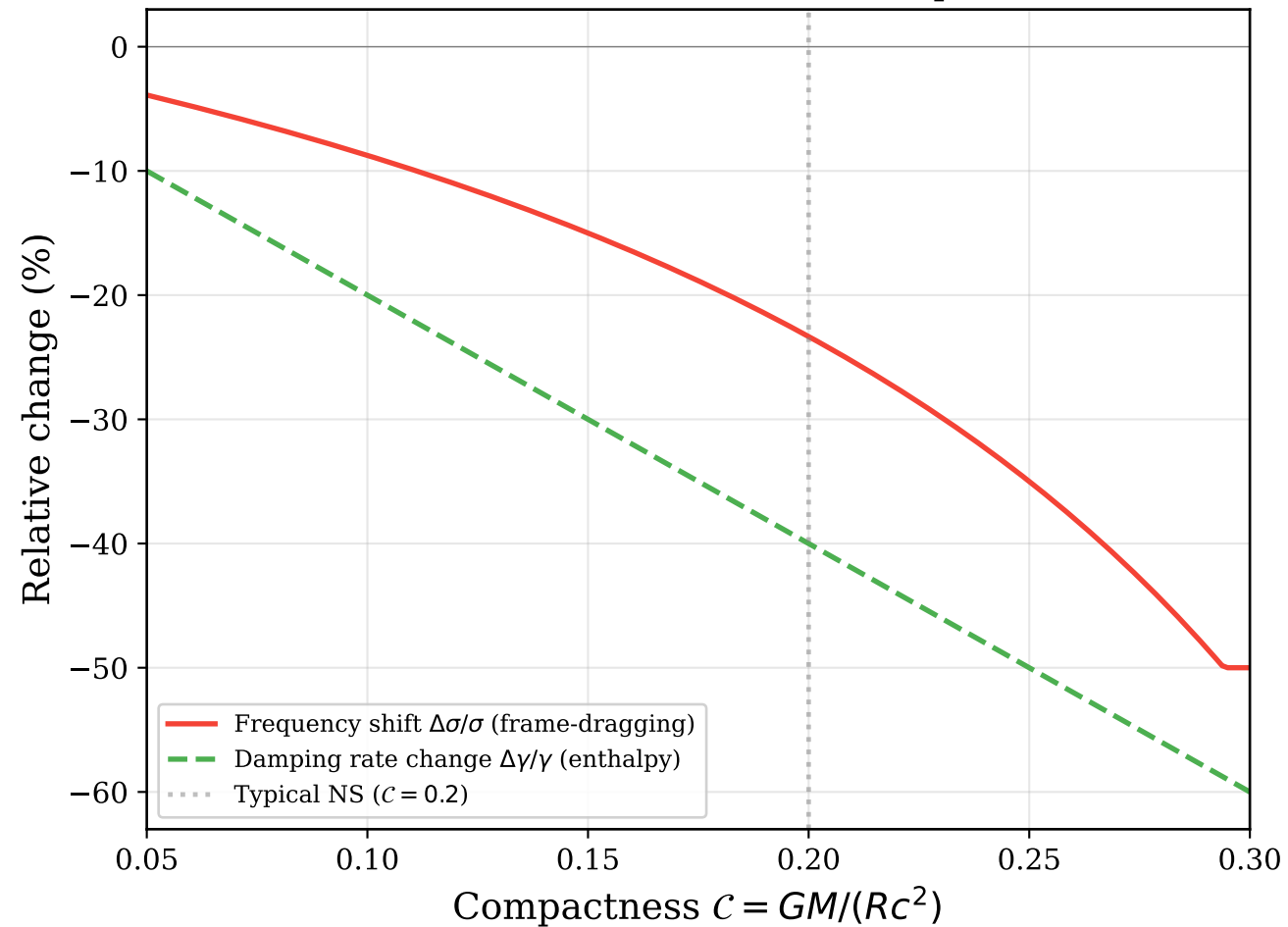
(b) Relativistic corrections vs compactness
