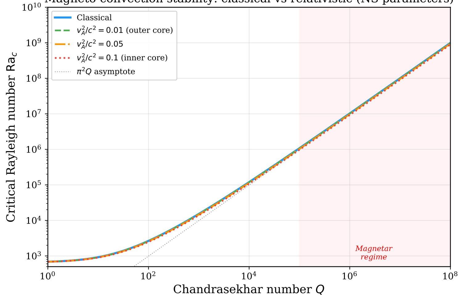
Magneto-convection stability: classical vs relativistic (NS parameters)
