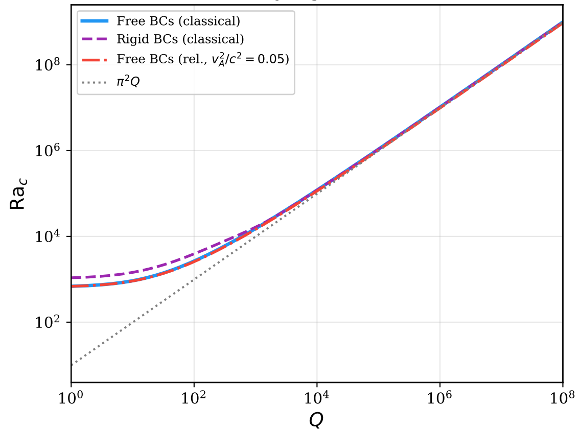
Critical Rayleigh number vs Q
