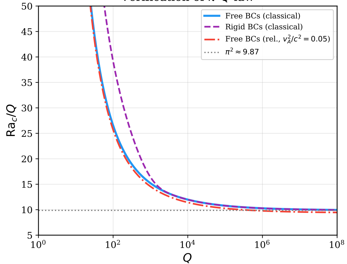
Verification of \pi^2 Q law
