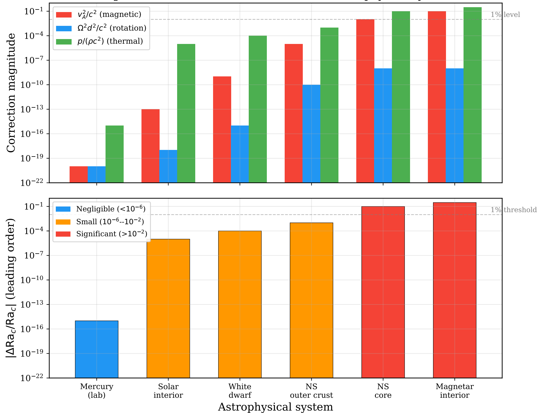
Magnitude of relativistic corrections across astrophysical systems
