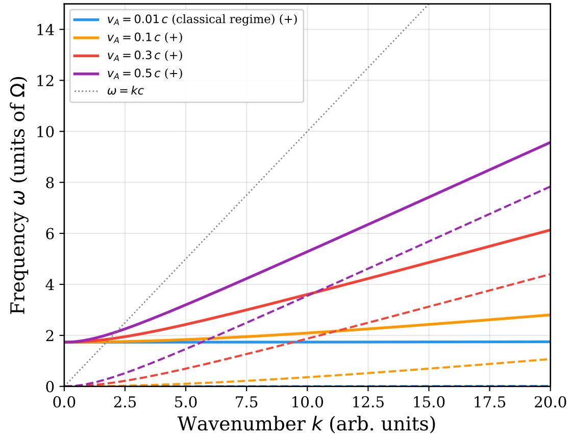
Magneto-inertial wave dispersion
