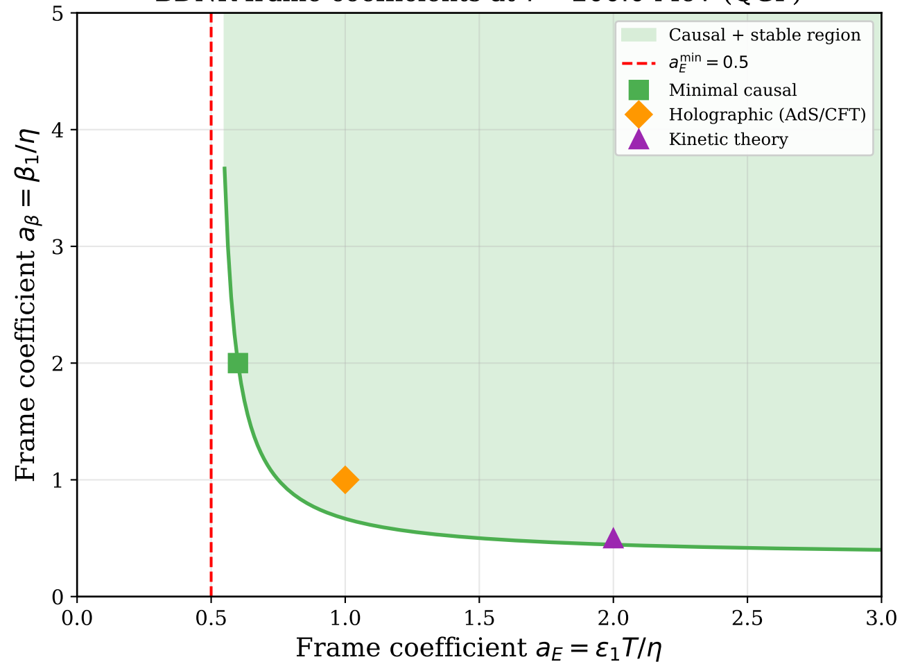
BDNK frame coefficients at T = 200.0 MeV (QGP)
