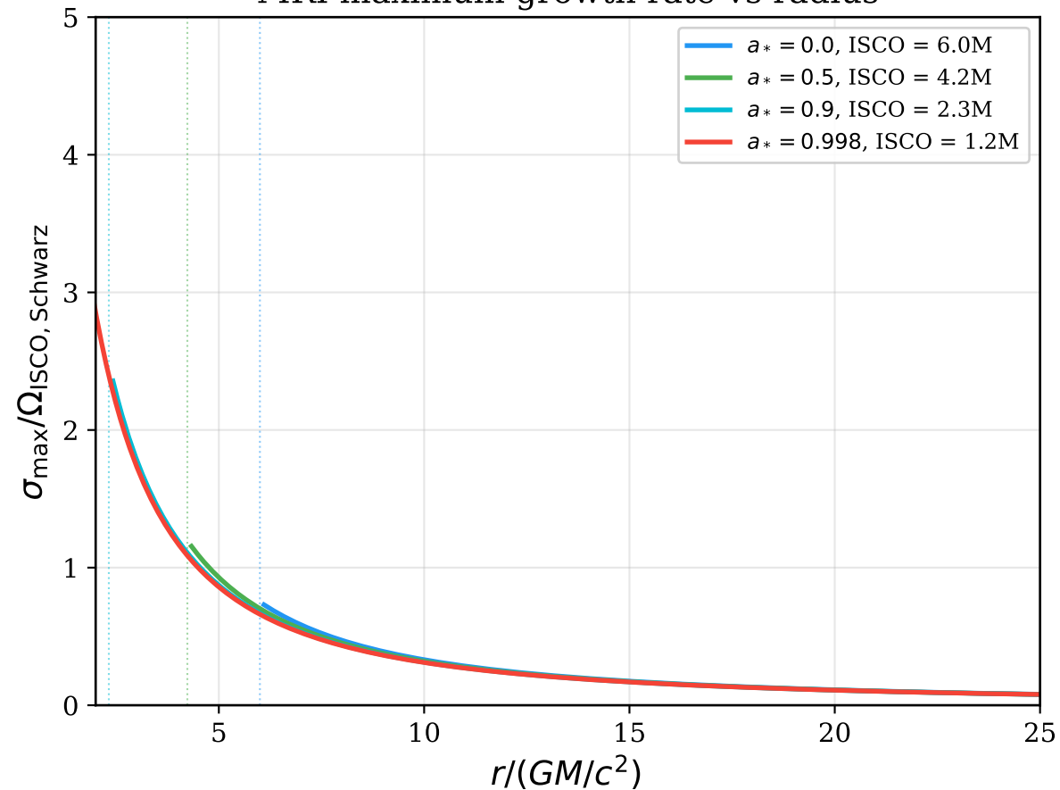
MRI maximum growth rate vs radius
