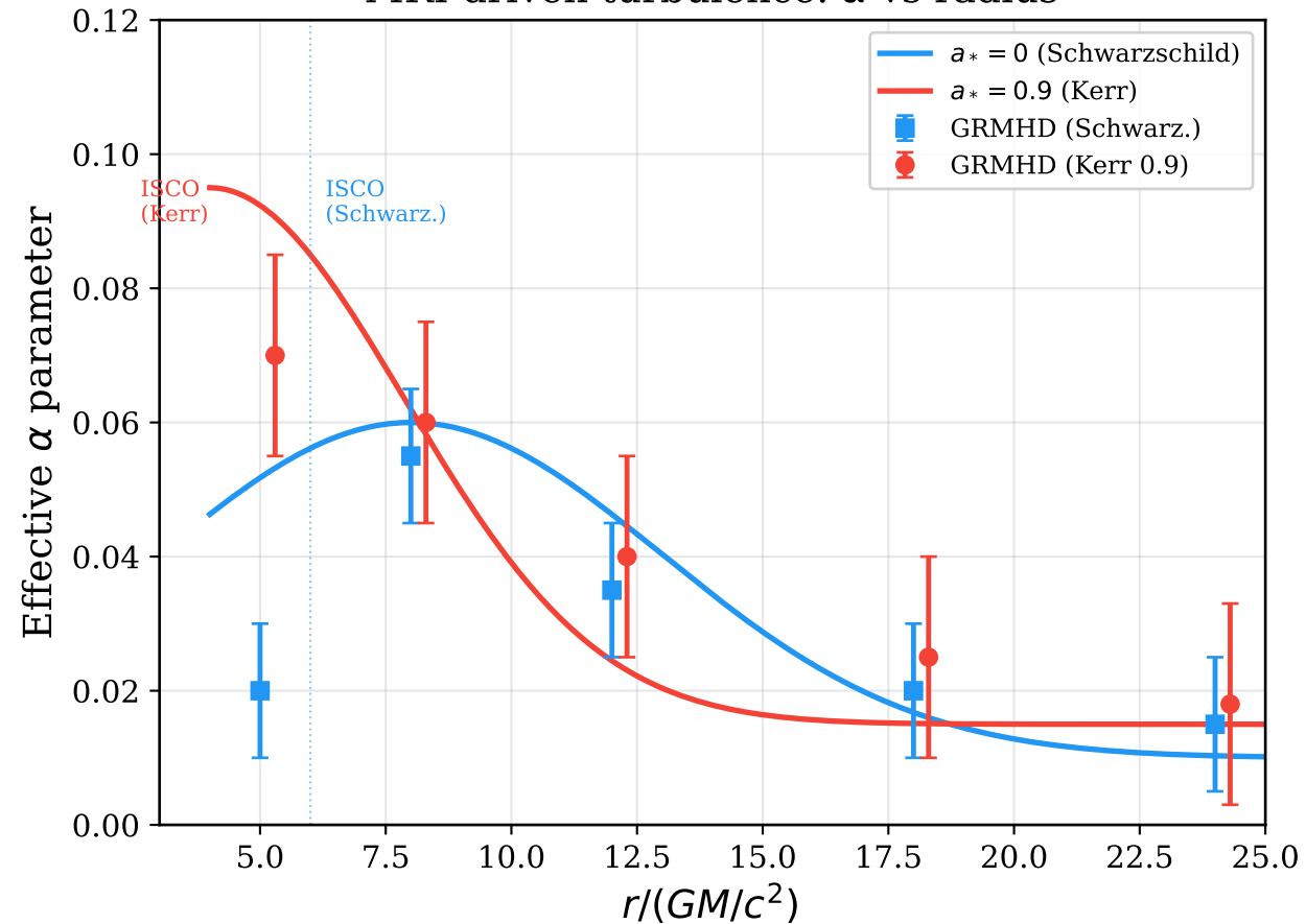
MRI-driven turbulence: \alpha vs radius
