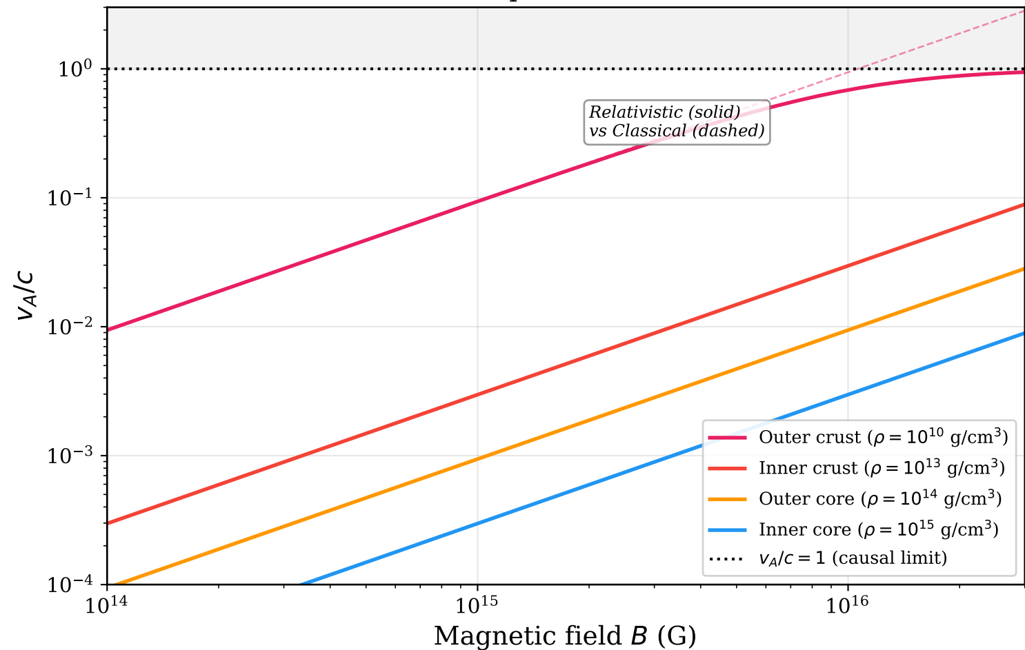
Relativistic Alfvén speed in neutron star interiors
