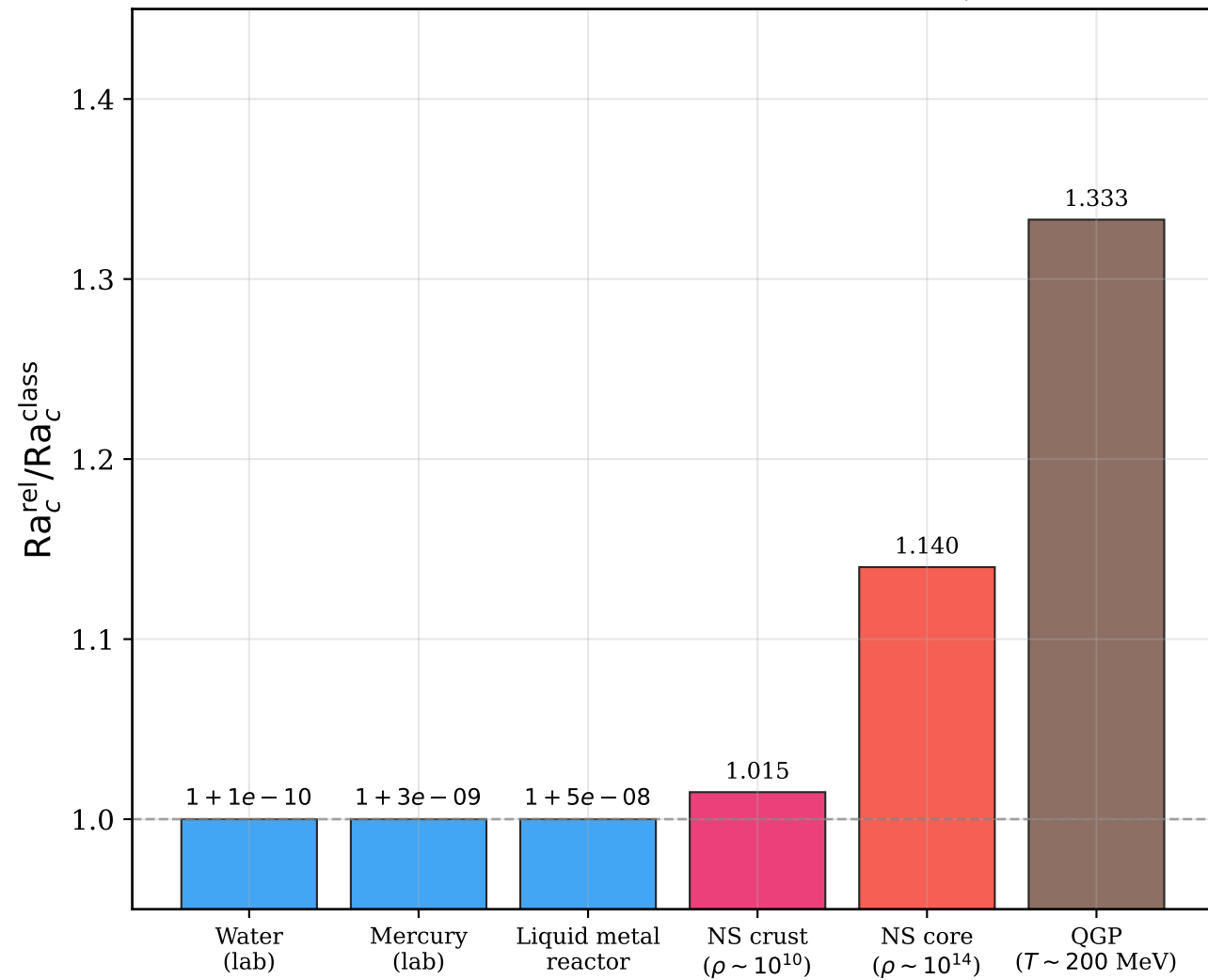
Relativistic correction factor (1 + \xi)
