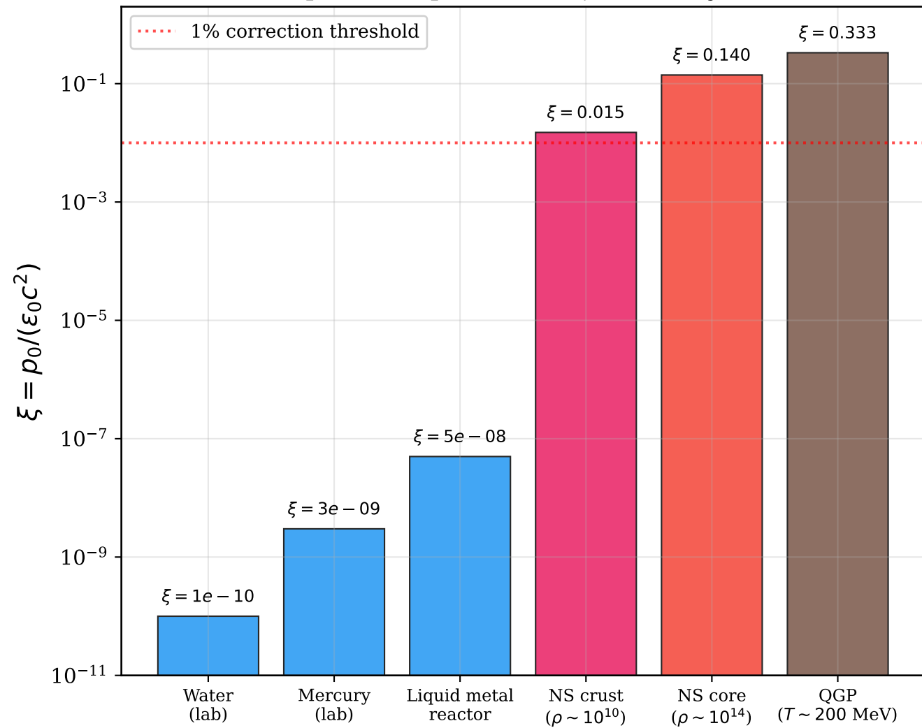
Compactness parameter \xi across systems
