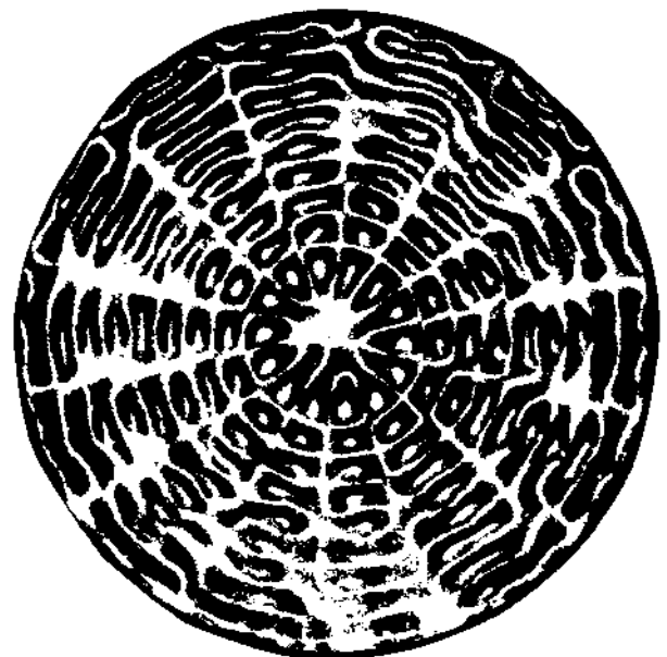
A Chladni figure formed by vibrating a sand covered disc to specific frequencies
