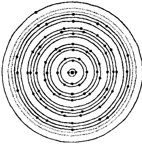
A flat representation of an atom of gold.
