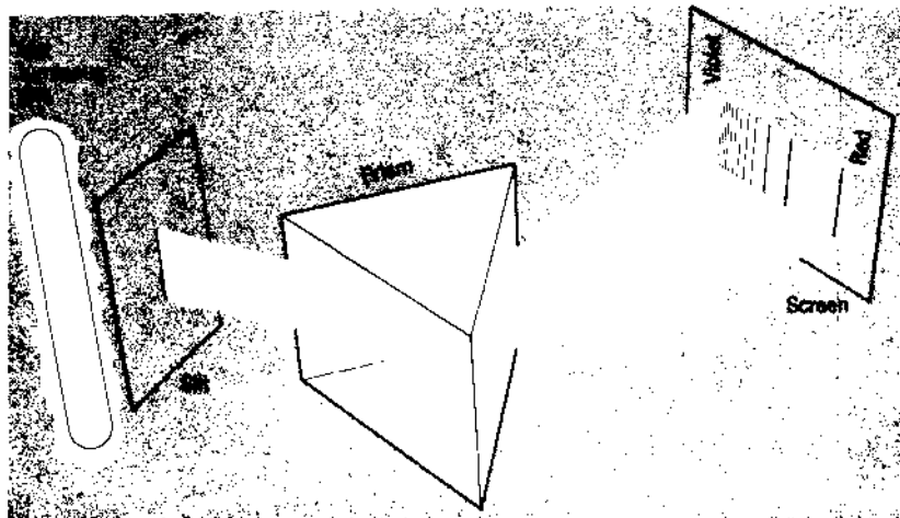
Line spectrum of a luminous gas.
