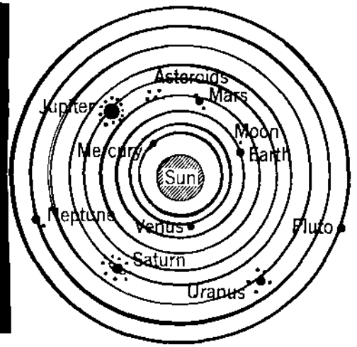
The Solar System. (These diagrams are not drawn to scale.)
