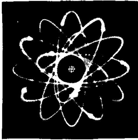
Artist's conception of an atom of oxygen.
