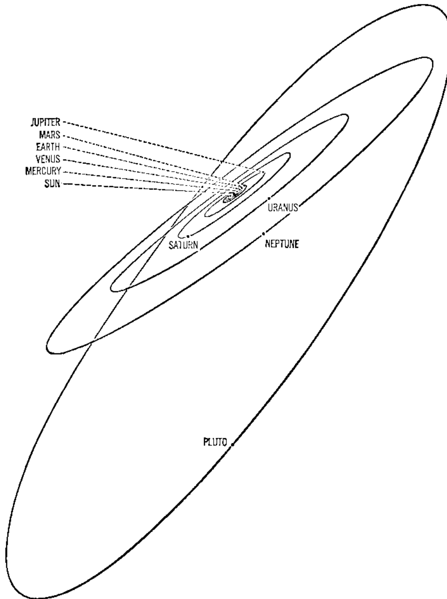
THE SOLAR SYSTEM, drawn schematically.
