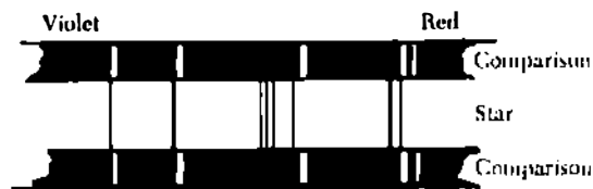
FIGURE (145) Doppler shift of stellar spectrum lines.
