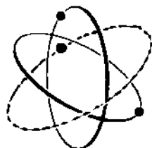
EXCITED NUCLEUS
