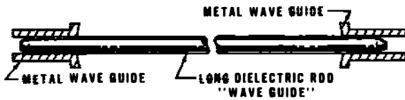
Fig. (266) A length of dielectric wave guide can connect two metallic wave guides.
