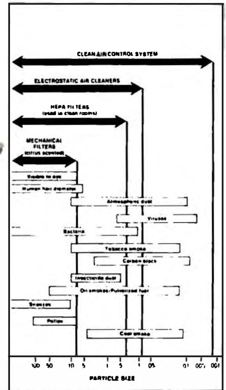
This chart illustrates the ability of the Ion Fountain Clean Air Control System to pull pollutants out of the air.
