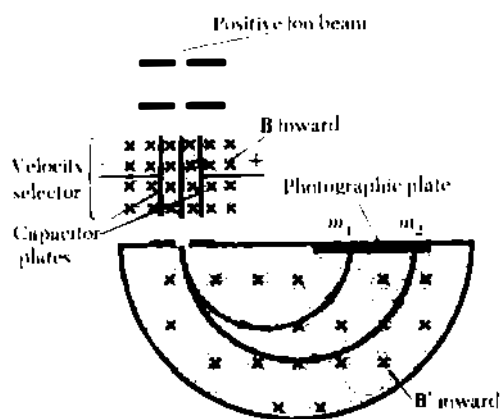
Fig. 196B The Bainbridge mass spectrometer (schematic).
