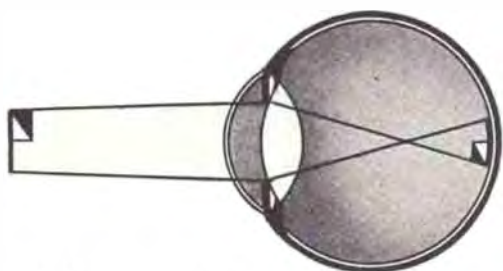
FIG. 130 The lens system of a nearsighted eye has high refractive power; it bends rays together easily. Therefore, the diverging rays from a near-by object are converged focused on the retina, and the result is a clear image. Notice that this image is upside down; to the brain, however, it is right side up.
