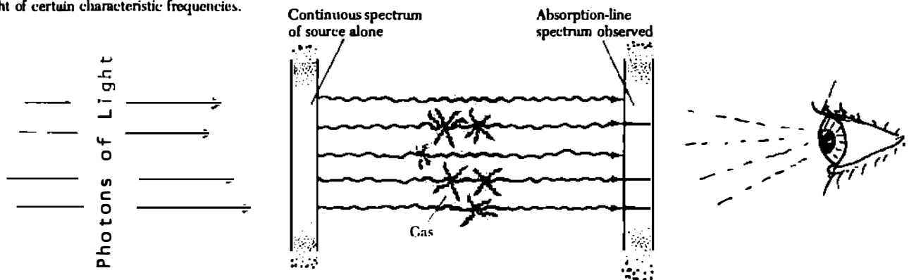
FIGURE (120) The dark lines originate when the cooler gas cloud absorbs light of certain characteristic frequencies.
