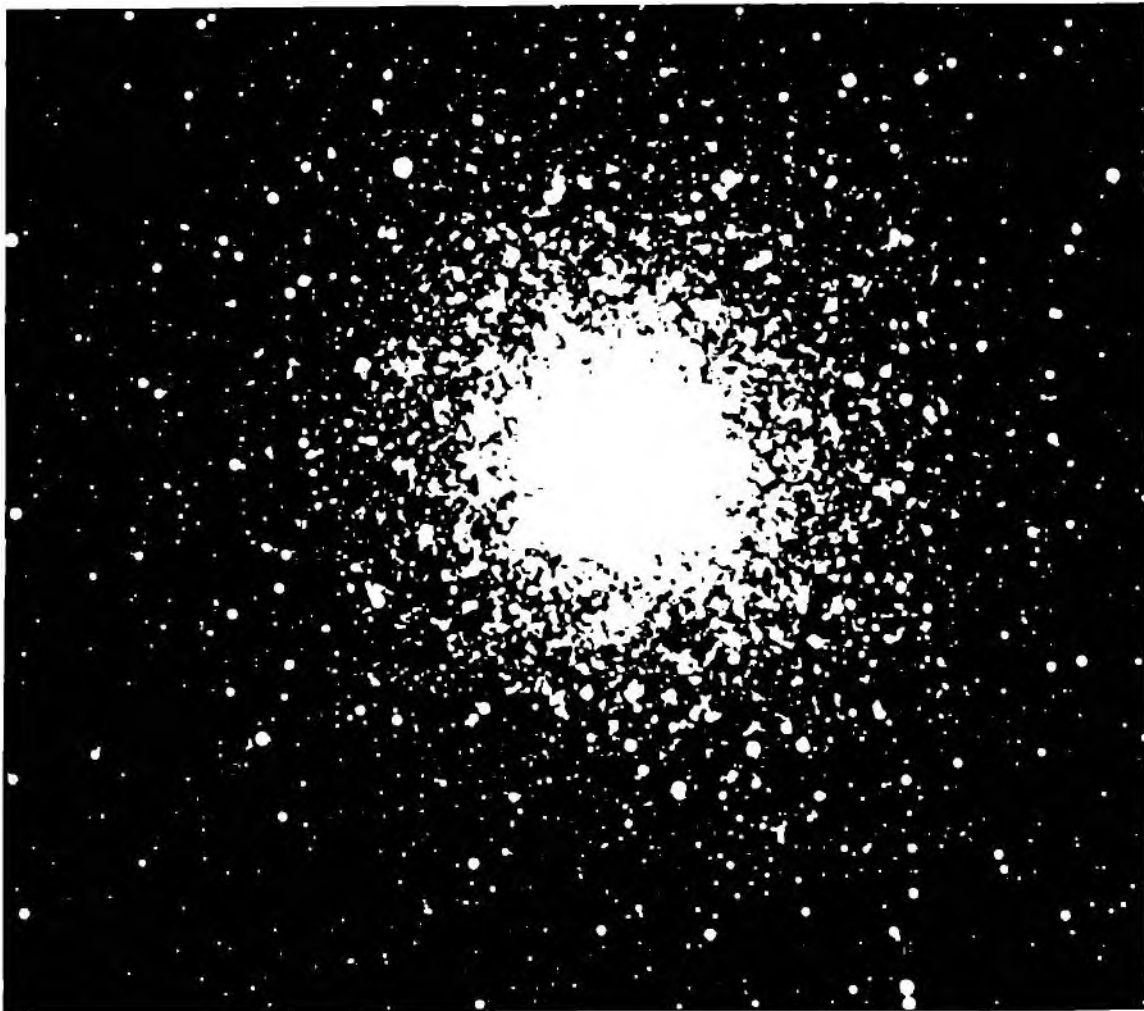
Fig. (126) Each star in this galaxy is a nodal point of energy vibration.. Each one radiating its spiral oscillating cosmic rays in all directions in the universal field. Light radiation in space is travelling in every direction at once, each star exchanging its own radiation with each other. Every person functions as a star but in a different harmonic octave. The nodal points of cosmic wave trains are about 6/1000ths of 1 mm apart whereas for humans they are about 13-80 cm.
