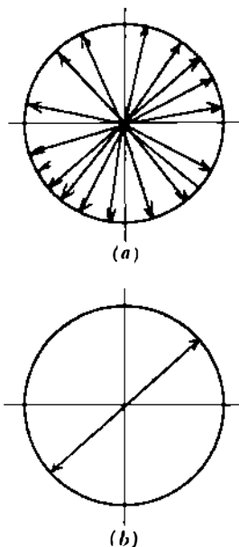
FIGURE (246) The structure (diagrammatic) of a beam of light. In ordinary, unpolarized light the vibration vectors lie in random directions around the line of propagation as in (a). If the vibrations are confined to just one direction, the light is plane-polarized, as shown in (b).
