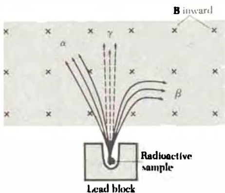
FIGURE 66 Effect of a magnetic field on the three types of rays from radioactive materials (schematic). Similar effects would be produced by an electric field directed toward the left in the figure.
