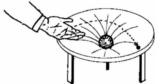
FIGURE(200) Visualizing the warping of space produced by the presence of a massive body. A marble rolled across a tightly stretched rubber membrane follows a straight path, but if a heavy object distorts the rubber sheet the marble will be deflected on passing by.
