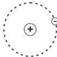
Fig. 66–Simplified model of atom
