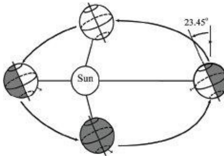
Fig. 96 – Earth orbit around the sun
