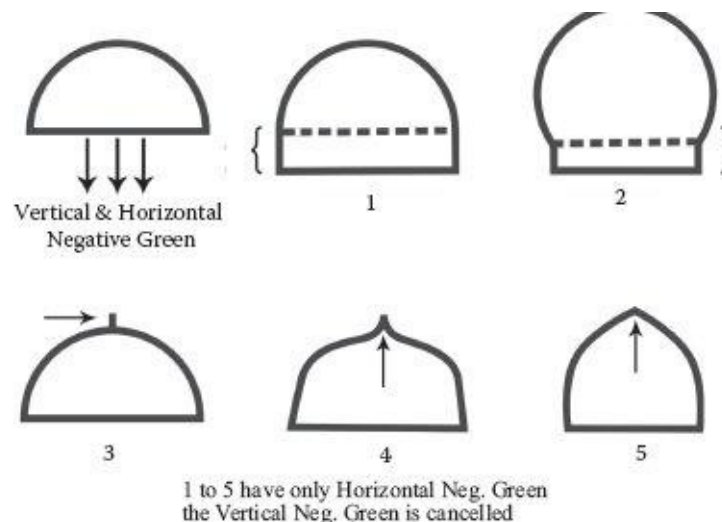
Fig. 33 – Dome solutions
