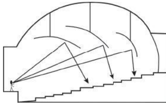
Fig. 2 - Theater acoustics
