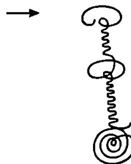
General Balance - Human-Earth-Solar Link
