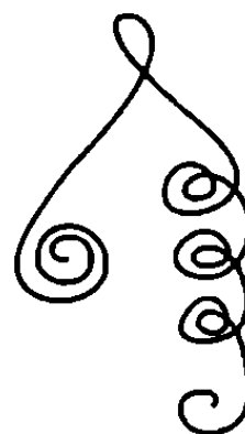
Fig. 23-1. Clearing Body Earth Radiation
