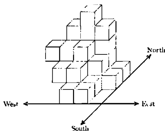
Fig.8 The Benker Cube System
