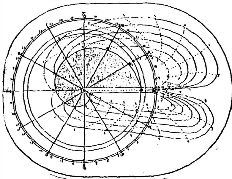
Figure 47. Perfected snail-disk.
