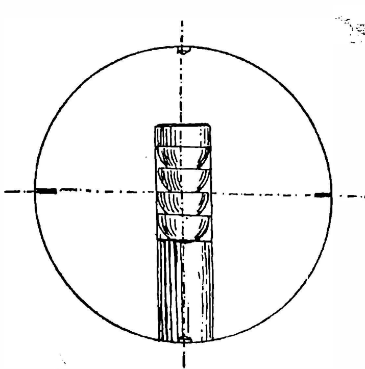
Figure 28. Cutaway view inside a pendulum stabilized by four elements.
