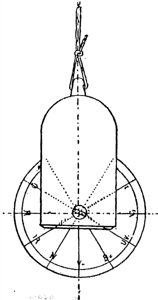
Figure 34. Pendulum with colorimetric disk, emitter-receptor.
