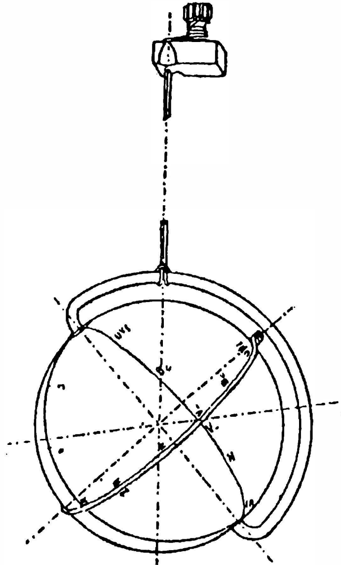
Figure 24. Placement on the Universal Pendulum of the non-magnetic metallic handle, permitting exploration of all the points on the sphere.
