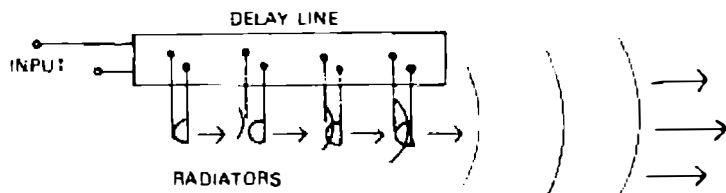
END-FIRE ARRAY ANALOGY WITH MODERN MICROWAVE GUIDE
