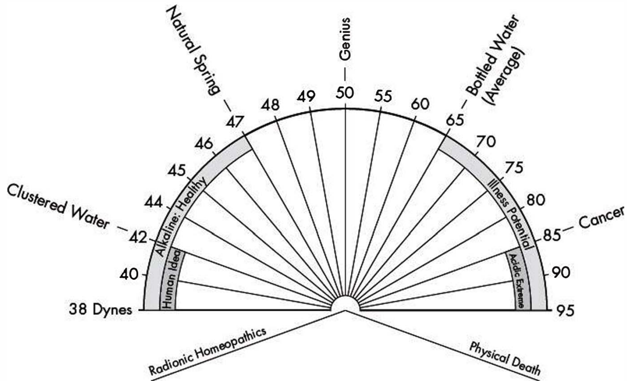
Chart 14. Water Surface Tension
