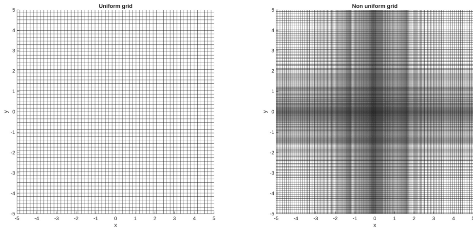
Figure 3.7.: Grid comparison
