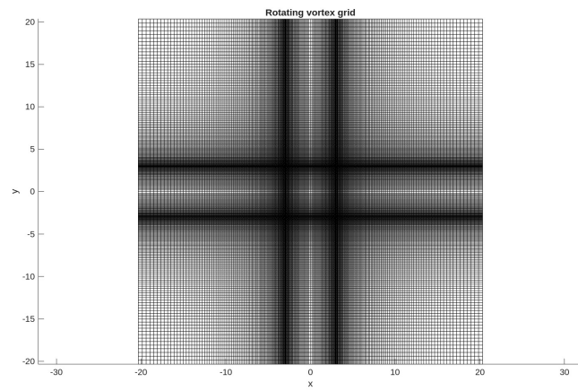
Figure 3.14: Grid used for rotating vortex simulation
