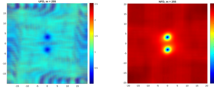
Figure 3.11: Comparison between equispaced grid and grid 3.14
