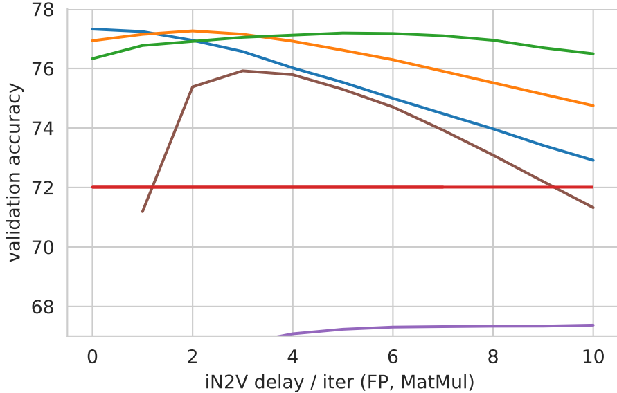
dataset = WikiCS
