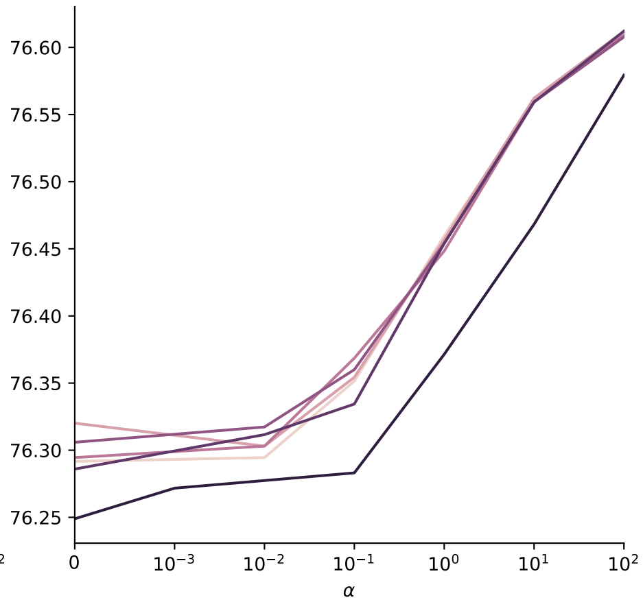
dataset = WikiCS
