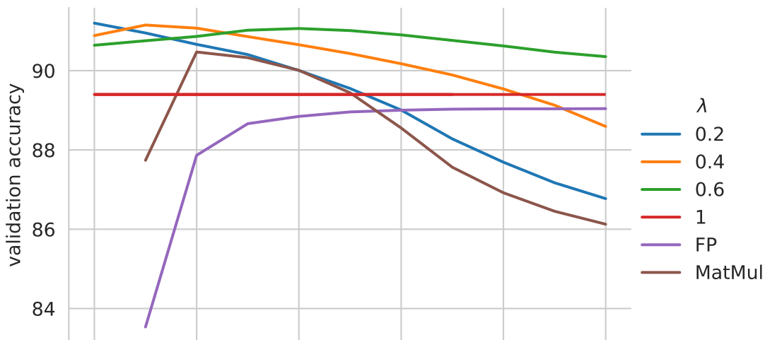
dataset = WikiCS
