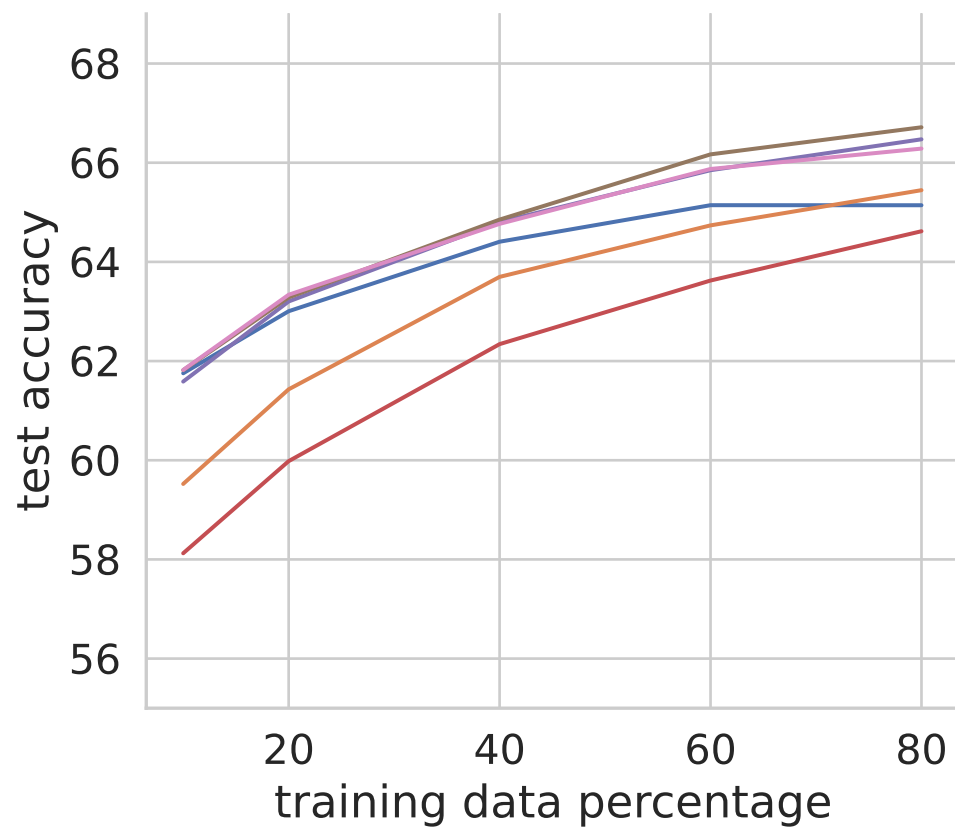
model = MLP
