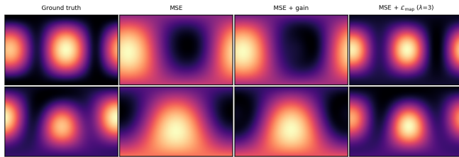
Fig. 2. Whole-clip energy maps ( 2^\circ equirectangular grid) for two test clips chosen where the map-loss model gains most over MSE: ground truth, MSE, MSE with the selected axis gain, MSE + \mathcal{L}_{\text{map}} . The gain sharpens the MSE map but cannot move its mass.
