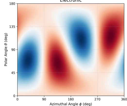
Bilinear Coupling
