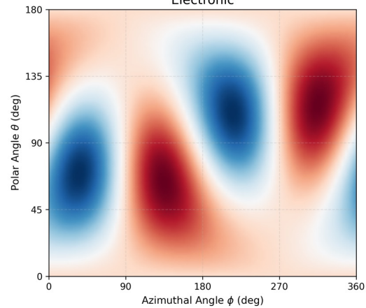
Energy-Component Decomposition: Ortho – Meta [Nel_49_Nph_10]
