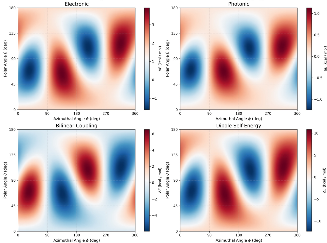
Energy-Component Decomposition: Ortho – Meta [NeI_49_Nph_4]
