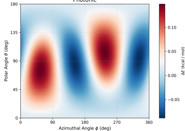
Dipole Self-Energy
