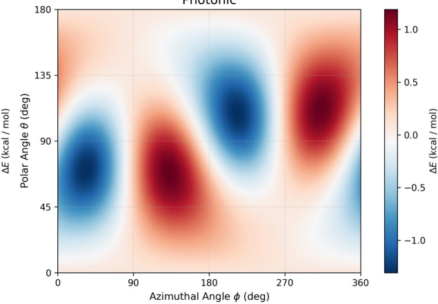
Energy-Component Decomposition: Ortho – Meta [Nel_49_Nph_10]
