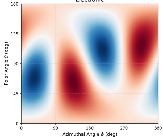
Energy-Component Decomposition: Ortho – Meta [Nel_49_Nph_3]
