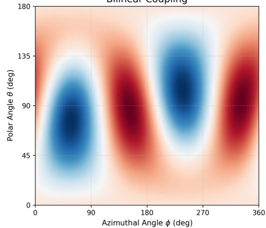
Bilinear Coupling
