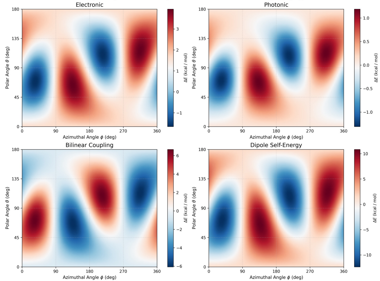
Energy-Component Decomposition: Ortho – Meta [NeI_49_Nph_10]
