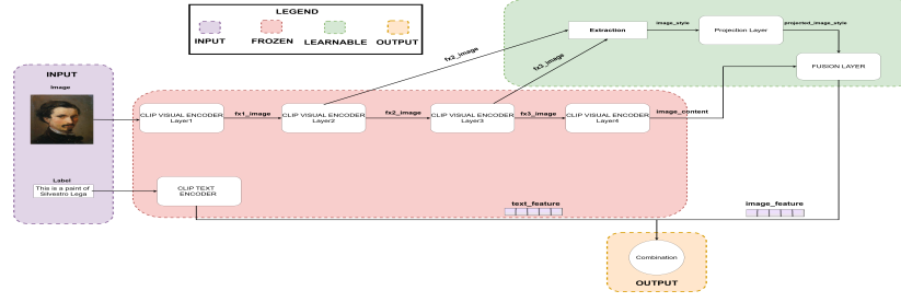
Figure 1: StyCLIP Architecture Overview
