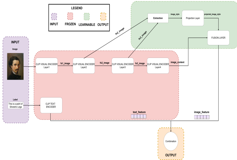
Figure: StyCLIP Architecture Overview
