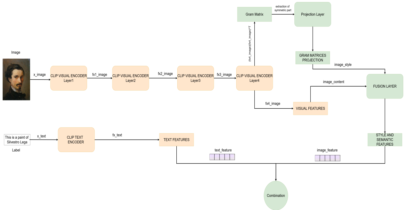
Figure 1: StyCLIP Architecture Overview
