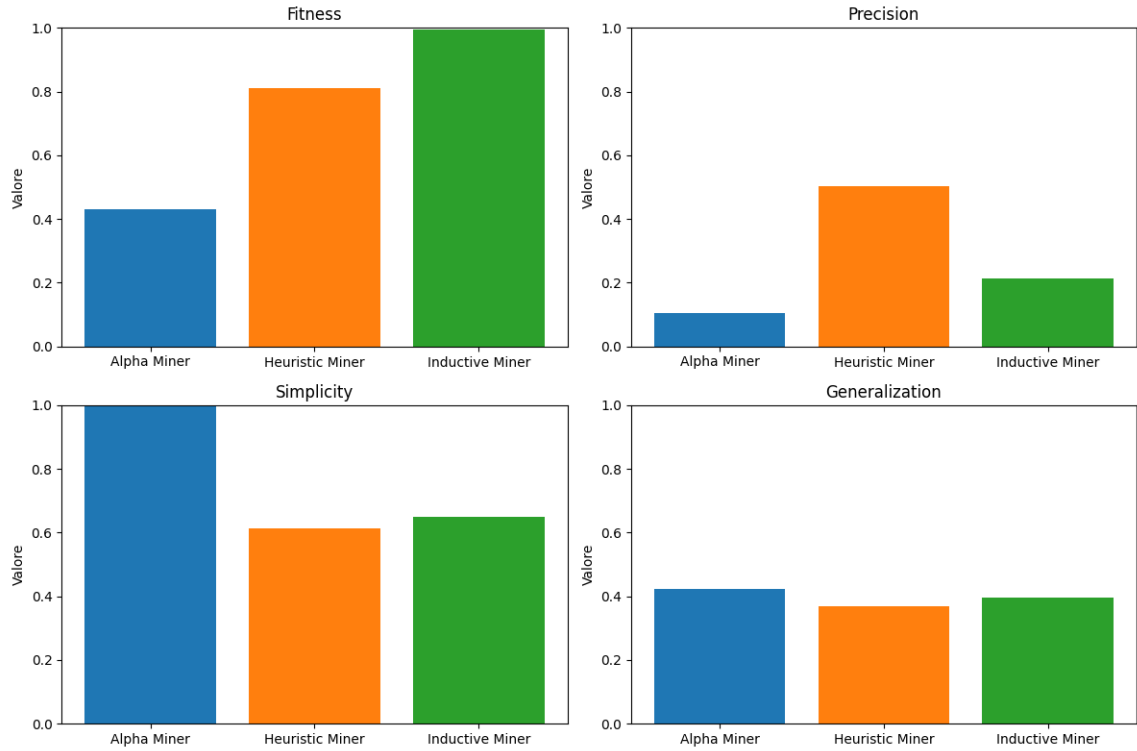
Figura 10: Performance metrics of the process mining algorithms
