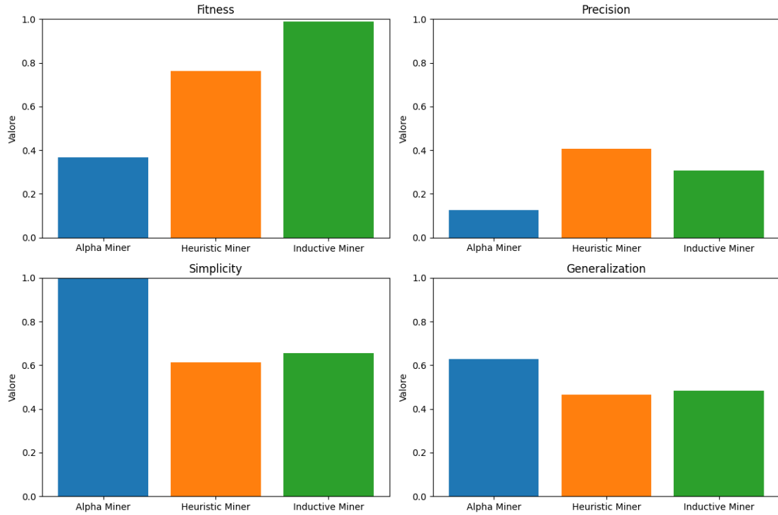
Figura 15: Performance metrics of the process mining algorithms
