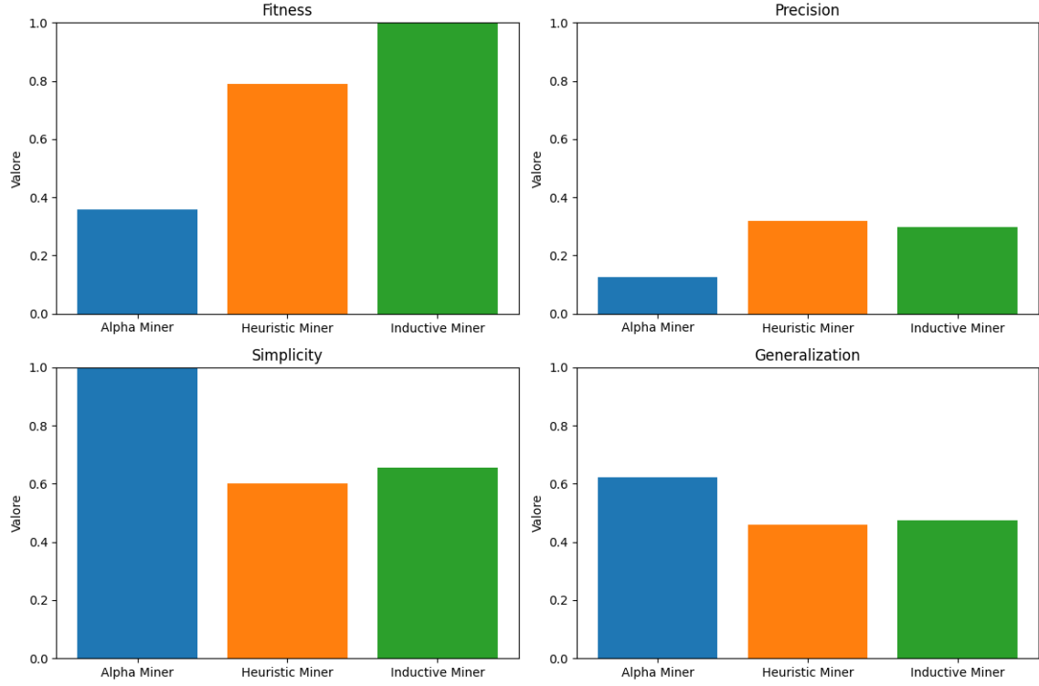
Figura 20: Performance metrics of the process mining algorithms
