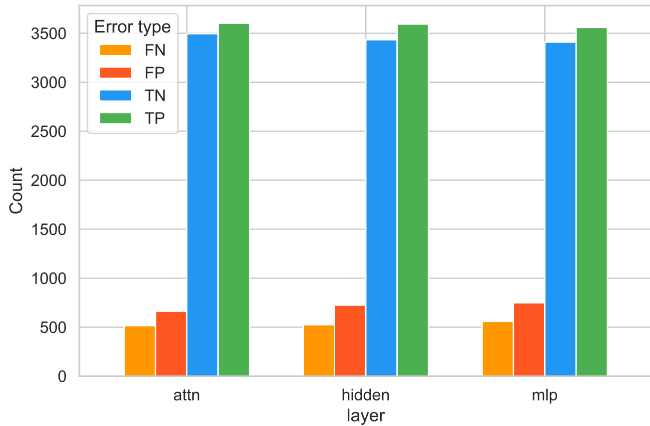
Llama-3.1-8B-Instruct
