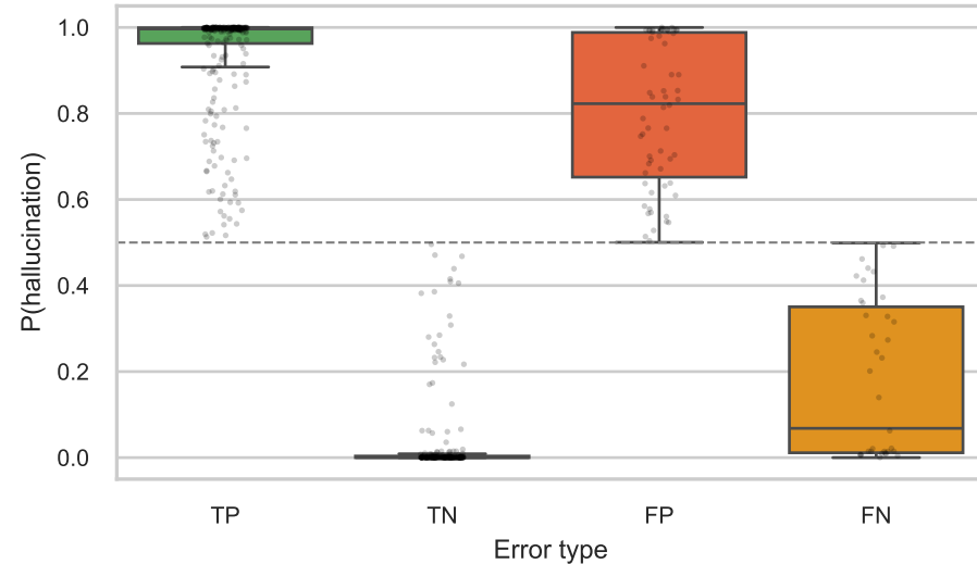
Llama-3.1-8B-Instruct
