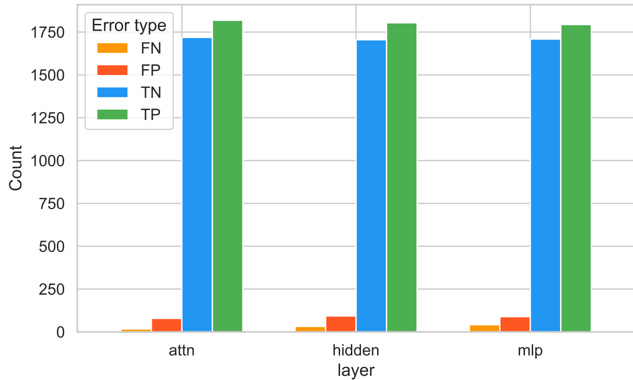
Llama-3.1-8B-Instruct
