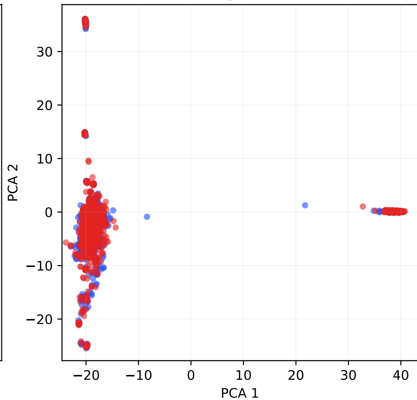
HaluEval (Layer 1)
