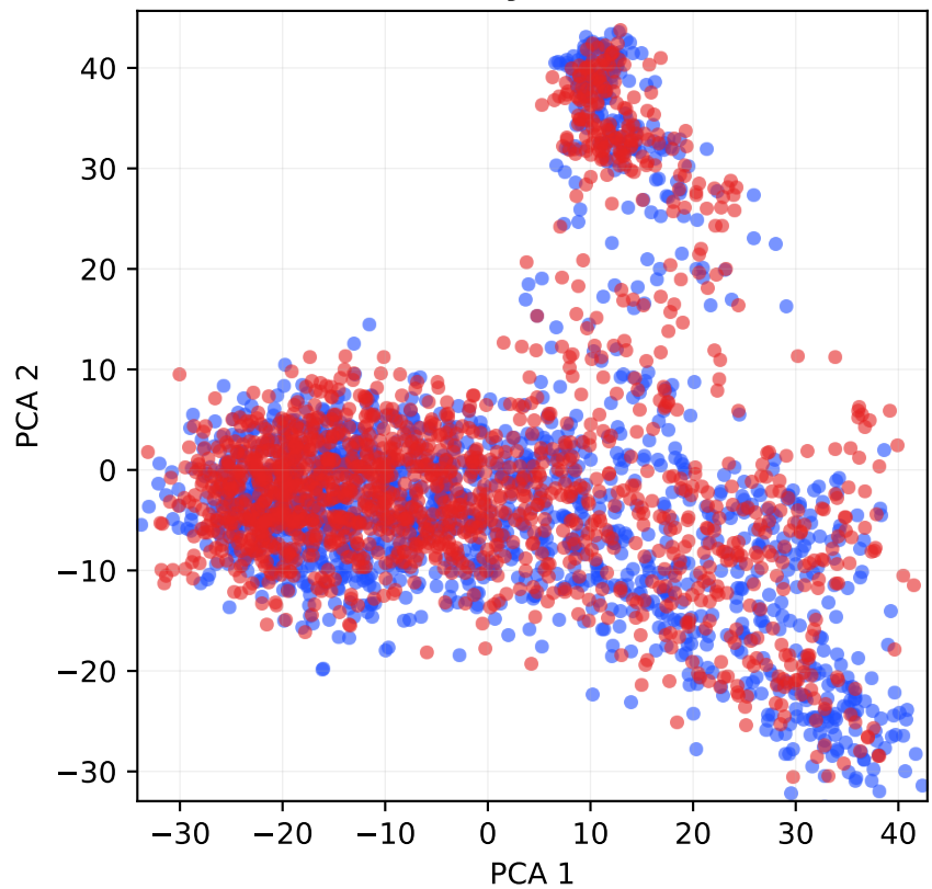
HaluEval (Layer 8)
