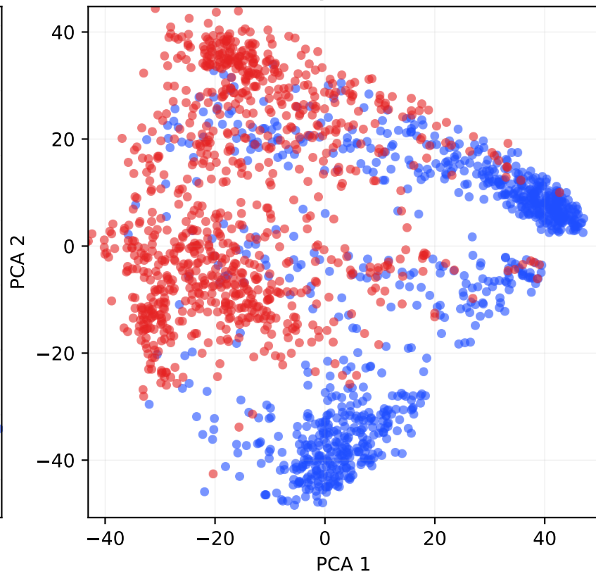
Belief Bank Facts (Layer 23)
