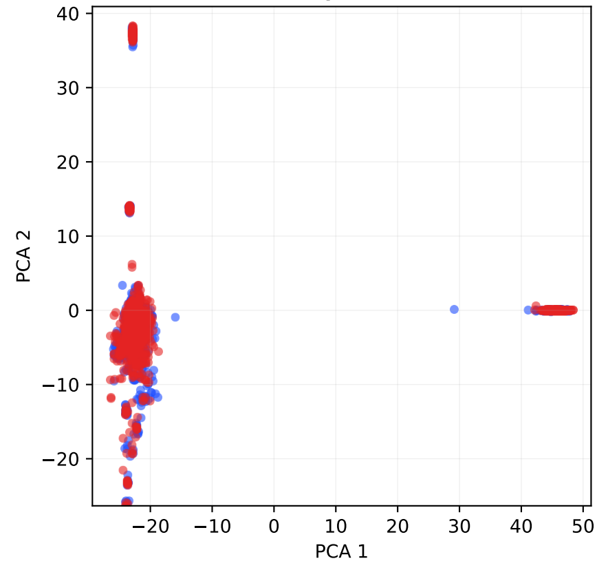
HaluEval (Layer 1)
